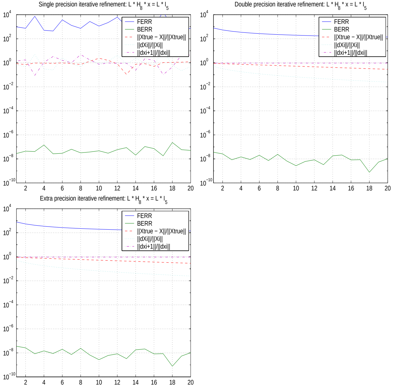
Figure 3: Iterative refinement results in Single, Double and Extra precision, n = 8, j = 5 .
