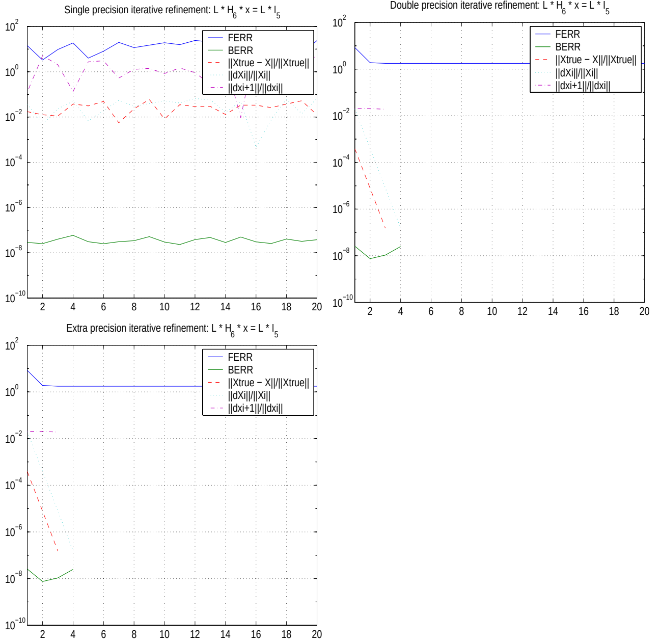
Figure 1: Iterative refinement results in Single, Double and Extra precision, n = 6, j = 5 .
