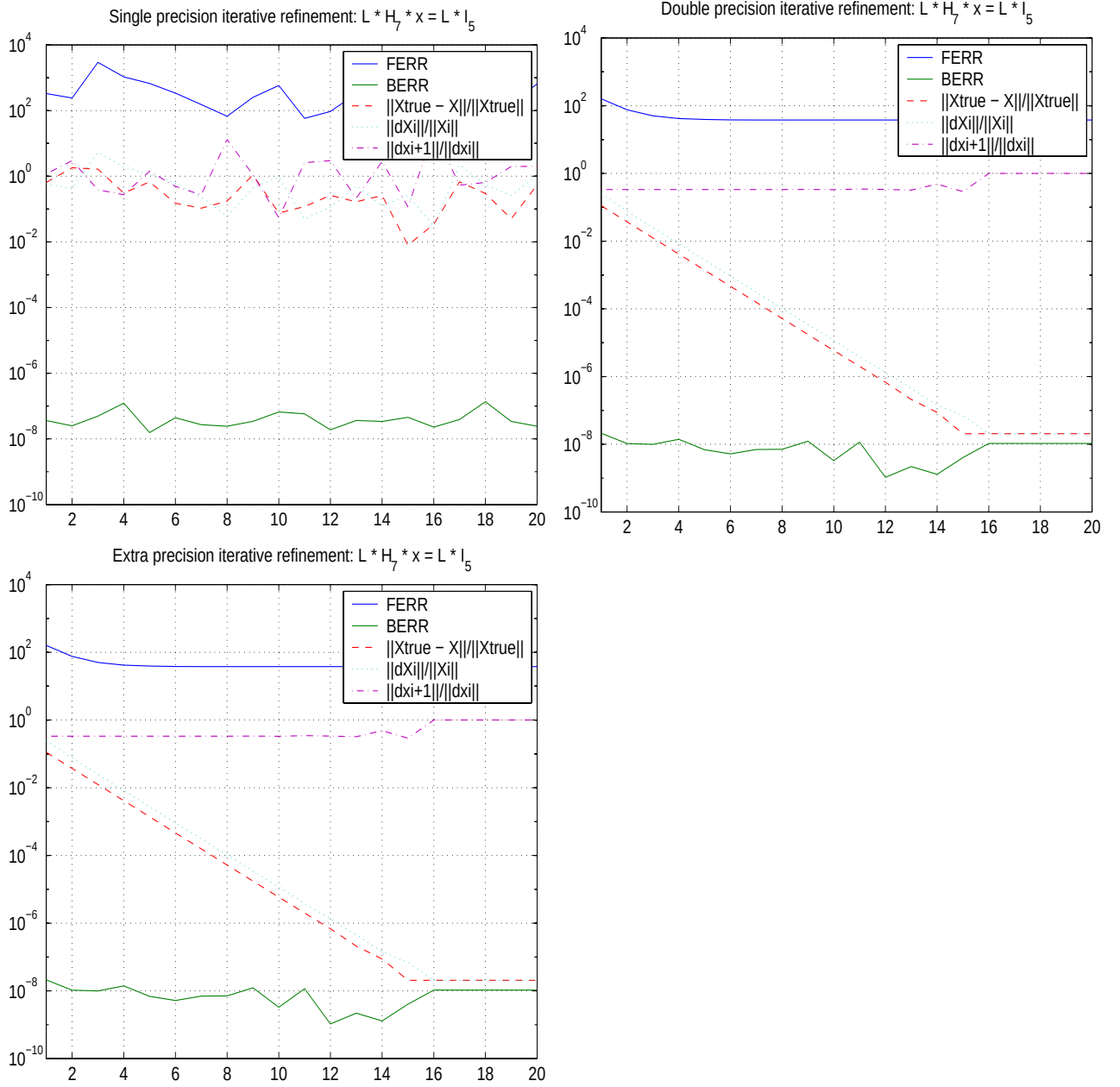
Figure 2: Iterative refinement results in Single, Double and Extra precision, n = 7, j = 5 .
