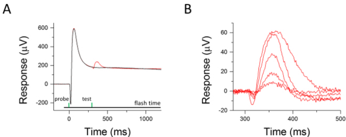
Figure 3. Isolation of cone responses with double flash method in WT mouse. (A) A response to probe flash (14,000 photons \mu\text{m}^{-2} or 1 dB green light, black) and a response to probe flash followed by a test flash (81,000 photons \mu\text{m}^{-2} or 9 dB green light, red). (B) Cone flash responses to test flashes ranging from 360 to 81,000 photons \mu\text{m}^{-2} (-14 to 10 dB green light) isolated by subtracting the probe flash response from the "probe + test flash" response. Please click here to view a larger version of this figure.
