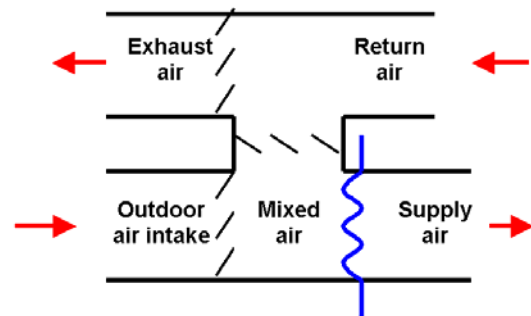
Figure 2. Air-side Economizer
