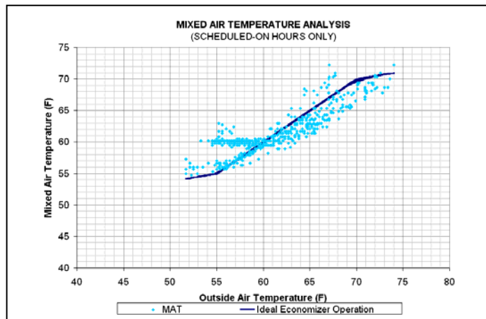
Figure 7. Tool A, Economizer Plot
