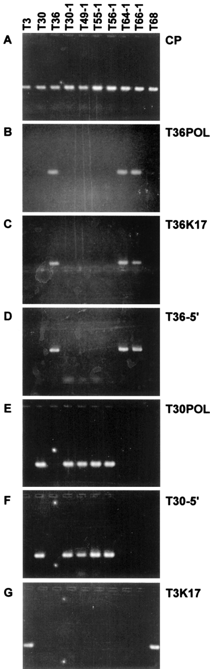
Fig. 3A-G. PCR amplification products from Florida isolates. The individual isolate is indicated at the top of the figure, and the marker amplified in each panel is indicated to the right. Lanes contain ethidium bromide stained DNA amplified from cDNA of the indicated isolate with the primer pair specific for the indicated marker. Figure 3 was published previously in Hilf et al. (4) and is used here with permission.
