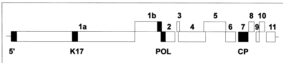
Fig. 2. Schematic diagram of the CTV genome based upon the T36 isolate. The viral open reading frames are indicated by numbers, and are listed in ascending order from the 5' to the 3'-terminus, in the manner of Karasev et al. (5). The approximate genomic locations of the sequence specific markers are indicated by shaded areas and by the name of the amplified marker. Figure 2 was published previously in Hilf et al. (4) and is used here with permission.
