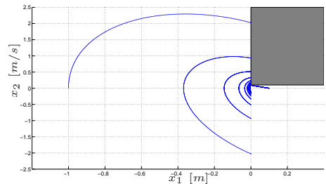
Fig. 4. Planar plot of the position and velocity trajectories (blue line) of the point mass. The gray box denotes the union of the flow set and jump set.
