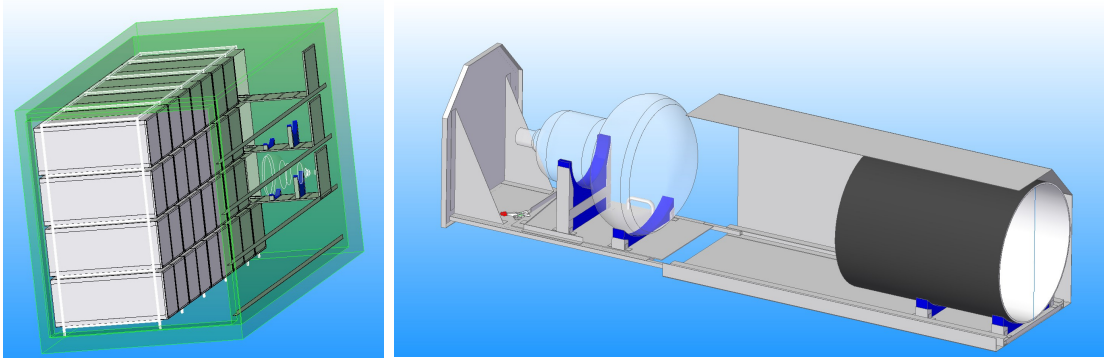
Figure 17: Left: Conceptual picture of the container with the shelf system including 36 drawer boxes. Right: Schematic view of the final design of the drawer system (for illustrative reasons one side of the drawer box is not depicted).
