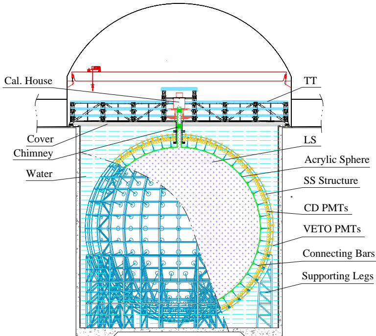
Figure 3: Schematic view of the JUNO detector
