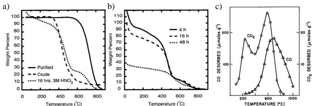
Fig. 19: (a,b) Normalized TGA spectra for SWNTs produced by laser ablation and then purified by a 2-step technique of acid reflux and air oxidation. After purification, the SWNT fraction resists oxidative weight loss up to 550 °C and has an inflection point at 735 °C (a). Acid reflux durations exceeding 16 hours are more effective at removing amorphous carbons, but a substantial reduction in SWNTs is also seen (b). (c) By coupling TGA with mass spectrometry, oxygen-containing functional groups may be titrated from acid-oxidized graphitic carbons. (b) Reproduced with permission from (Dillon et al., 1999). Copyright 1999 Wiley-VCH. (c) Reproduced with permission from (Barton et al., 1973). Copyright 1973 Elsevier Limited.
