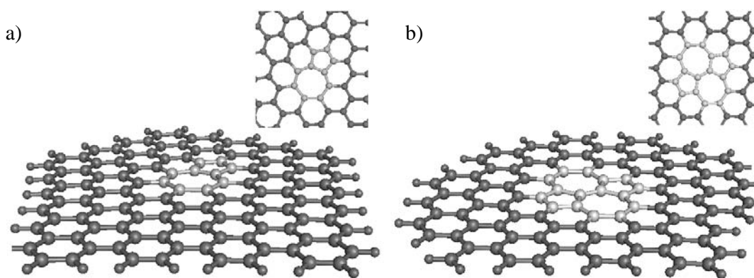
Fig. 2: (a) A single 5-7 defect and (b) a 5-7-7-5 Stone-Wales configuration. Sighting along the zigzag edges in a side view visualization clarifies the nucleation of a dislocation by the 5-7 defect, and the absence of long-range disorder in the Stone-Wales case.
