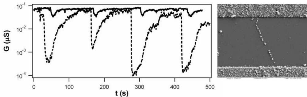
Fig. 25: G(t) for two SWNT sensor devices electrochemically decorated with Pd, as they are repeatedly probed by H_2 gas in air. G decreases \sim 40\% in the first device (solid line), a semiconducting SWNT liberally decorated as shown in the micrograph. G decreases more than 99% in the second device (dashed line), composed of a semi-conducting SWNT with a single, selectively-decorated defect. Reproduced with permission from (Khalap, 2008).
