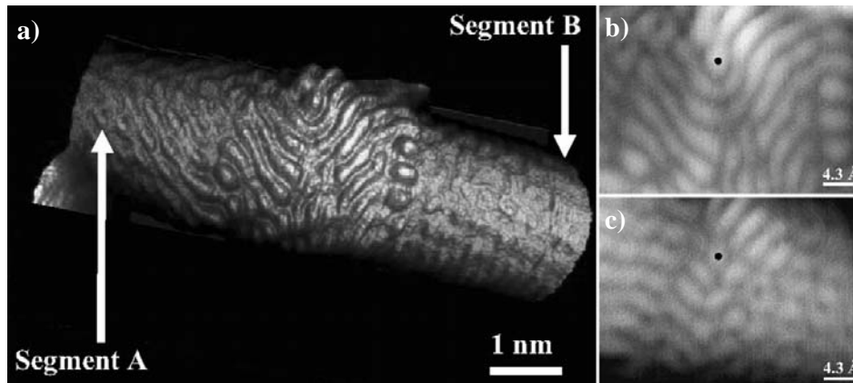
Fig. 7: (a) STM resolved point defect between two chirally-distinct segments in a 1.4 nm SWNT. The same location, as denoted by the black dot, appears different when imaged at different biases because of the complex electronic structure. Experimental conditions are 77 K, 0.2 nA, and +0.5 V (a,b) or +0.3 V (c). Continuous evolution of the image complicates any straightforward atomistic interpretation, but provides an extensive data set to compare against theoretical models. This site was determined to be a 5-7 defect, physically separated from a second 5-7 defect located on the hidden backside of the SWNT. Reprinted with permission from (Ishigami et al., 2004). Copyright 2004 American Physical Society.
