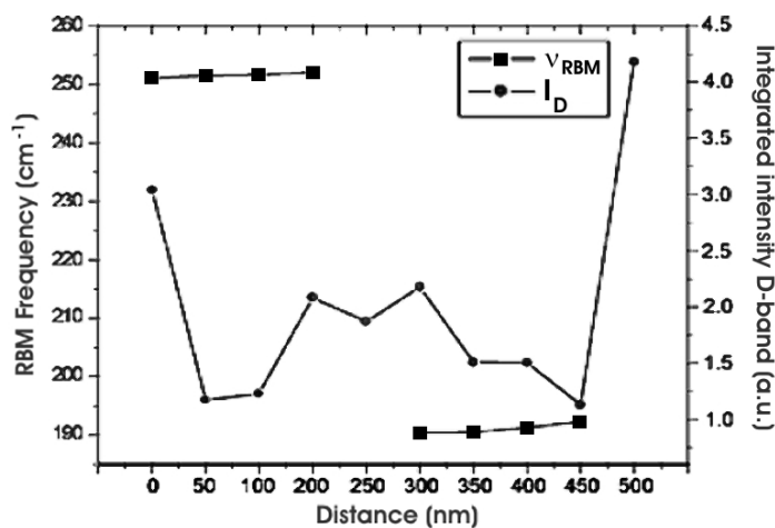
Fig. 15: Direct and indirect Raman spectroscopy of a defect in a single SWNT. The RBM mode abruptly shifts from 250 to 190 \text{cm}^{-1} (left axis), indirectly identifying a defect through its effect on the SWNT diameter. Within the transition region, the D-band intensity approximately doubles (right axis). Note that the D-band intensity is much higher at both SWNT ends, indicating one difficulty of resolving sidewall disorder. This apertureless measurement achieved 40 nm lateral resolution by using plasmonic-enhancement from a Au probe. Reprinted with permission from (Anderson et al., 2007). Copyright 2007 American Chemical Society.
