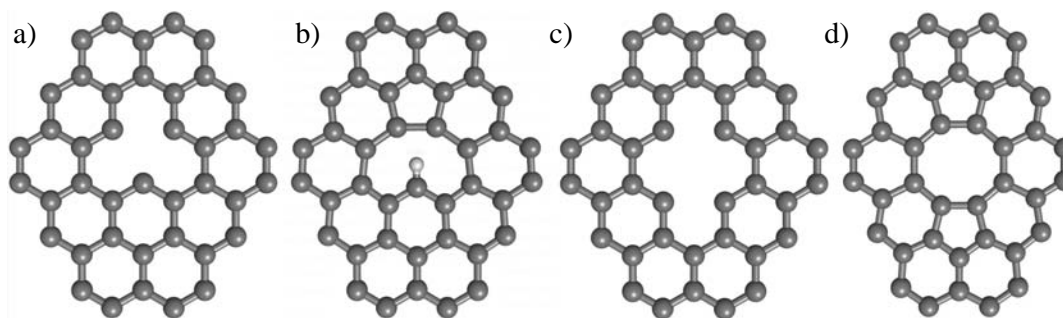
Fig. 1: Small vacancy defects in the graphene system. Mono-vacancy (a) before and (b) after reconstruction and H-termination of the remaining dangling bond. Di-vacancy (c) before and (d) after reconstruction.
