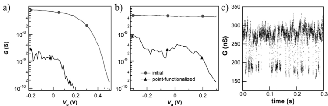
Fig. 24: A semiconducting (a) and a metal SWNT (b) both exhibit a reduced, gate-sensitive G following the incorporation of a carboxylate defect. Note that the gate voltage on the x-axis is applied to a liquid electrolyte. c) G fluctuations of 50% indicate ongoing binding dynamics between the carboxylate defect and a surrounding electrolyte containing EDC. Adapted and reproduced with permission from (Goldsmith et al., 2008). Copyright 2008, American Chemical Society.
