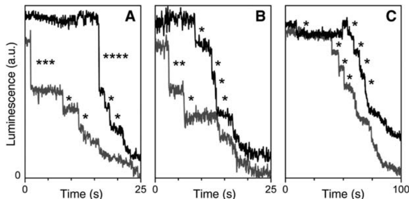
Fig. 16: Stepwise quenching of SWNT photoluminescence during the stochastic addition of covalent adducts, in this case 4-chlorobenzene-diazonium tetrafluoroborate. Each panel represents a different SWNT, with two curves for two adjacent, independently-measured segments (670 nm in length). Each asterisk indicates one unit of PL decrease. Adapted and reproduced with permission from (Cognet et al., 2007). Copyright 2007, American Association for the Advancement of Science.
