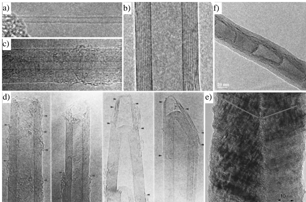
Fig. 4: TEM images of (a) a pristine SWNT, (b) a clean-walled MWNT, and (c-f) MWNTs with varying degrees of disorder. Layers of amorphous carbon, fullerenes, and mesoscopic graphitic sheets are common MWNT impurities. Lattice disorder includes (e) “herringbone” and (f) “bamboo” defects described in the text. (d) Reprinted with permission from (Iijima et al., 1992a). Copyright 1992 American Physical Society. (e) Reprinted with permission from (Park et al., 1999). Copyright 1999 American Chemical Society. (f) Reprinted with permission from (Jia et al., 2005), copyright 2005 Wiley-VCH.
