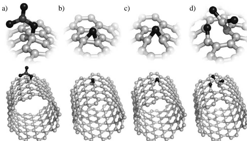
Fig. 3: (a) An adduct defect, in which the carbon lattice is not broken but a single atom is \text{sp}^3 hybridized, slightly puckering the CNT wall. Here an \text{NO}_3 adduct is depicted. (b) Stripping an adduct often leaves a residual oxygen, which binds two carbons in an epoxide configuration. The epoxide is stable on flat graphites or when its axis is parallel to the SWNT axis. (c) Along a circumference, the additional strain from curvature breaks the C-C bond in an epoxide, converting it to an ether. The ether is less perturbative because each carbon is \text{sp}^2 hybridized (Lee and Marzari, 2006). (d) A carboxylate defect is not an adduct. It requires cleavage of two C-C bonds, both of which must be terminated (-H or -OH groups not shown), and upon annealing a C atom is lost from the system. O atoms are black in all four images.
