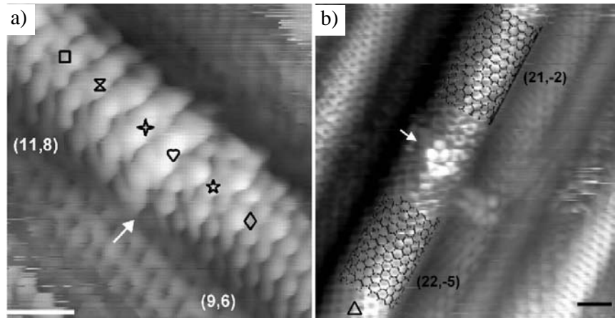
Fig. 6: In these examples, a change in chiral indices determines the presence of unpaired 5-7 defects. (a) At least two, separated 5-7 defects are present (i.e. not paired together in an SW configuration). (b) Three 5-7 defects are required to produce this change in chirality. Scale bar is 1 nm in both. Reprinted with permission from (Ouyang et al., 2001). Copyright 2001 American Association for the Advancement of Science.
