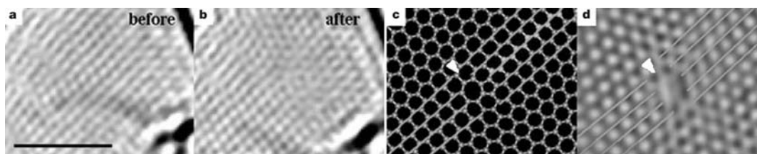
Fig. 9: Before (a) and after (b) TEM images of a single graphene layer with a beam-induced 5-7 defect. An edge dislocation is unambiguously visible at the middle of the network where one zig-zag chain is missing through it. (c) An atomistic model of the pentagon–heptagon pair in the graphitic network. (d) A simulated TEM image, showing good comparison with the TEM image shown in b. Scale bar, 2 nm. Reproduced with permission from (Hashimoto et al., 2004). Copyright 2004, Nature Publishing Group.
