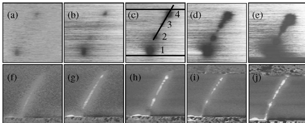
Fig. 18: SGM (a-e) and SIM (f-j) images taken at varying biases of a SWNT device with electrostatically-sensitive sites. Positions of the contact electrode interfaces are drawn in (c). Under some conditions, gating is solely observed at the Schottky barriers at both ends of the device (a,b). Additional inhomogeneity is observed with larger and more perturbative tip biases (c,d). Reproduced with permission from (Freitag et al., 2002). Copyright 2002, American Physical Society.
