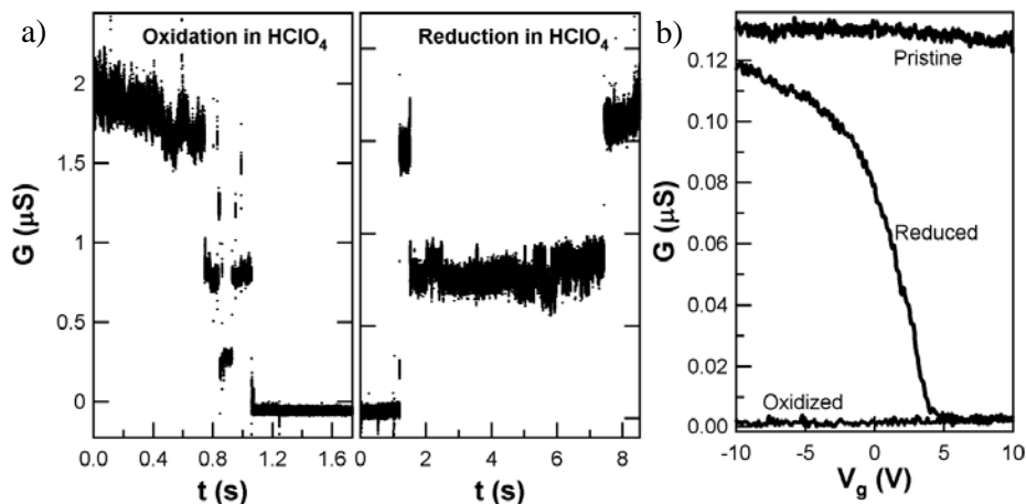
Fig. 23: a) G(t) during oxidative incorporation of adduct defects in \text{HClO}_4 , followed by electrochemical reduction of the same SWNT. Sharp steps of 10 – 30% are attributed to individual chemical events. b) G(V_g) for a metallic, pristine SWNT oxidized and then reduced. Substantial recovery of G following reduction is due to the formation of ethers, which have \text{sp}^2 conjugation and high conductance. Note that measurements are at low bias (100 mV), and that tunneling across the defect state dominates G at higher bias. Reproduced with permission from (Goldsmith et al., 2007). Copyright 2007, American Association for the Advancement of Science.
