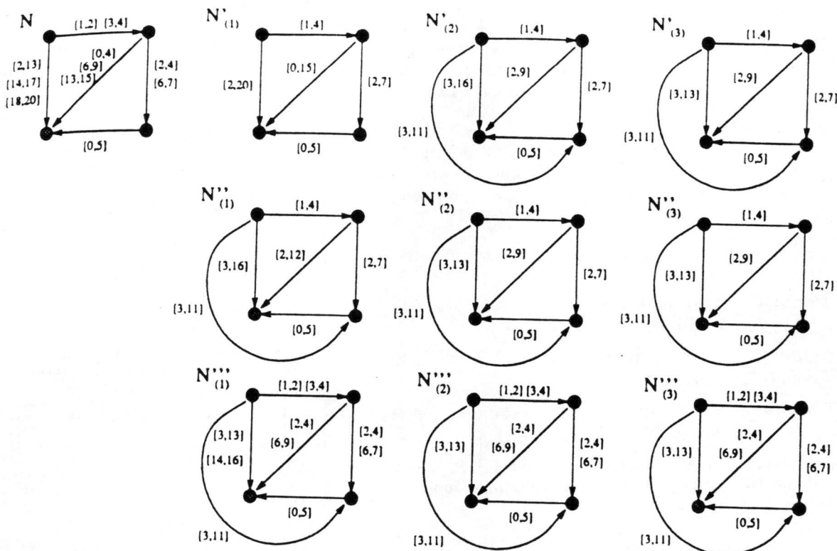
Figure 5: A sample run of ULT. We start with N (Figure 1) and compute N'_{(1)} , N''_{(1)} , N'''_{(1)} . Thereafter, we perform a second iteration in which we compute N'_{(2)} , N''_{(2)} , N'''_{(2)} and finally, in the third iteration, there is no change. The first iteration removes two intervals, while the second iteration removes one.
