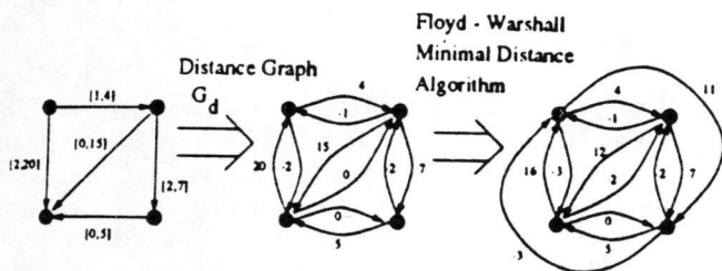
Figure 4: Processing an STP. The minimal network is in Figure 5, network N'''_{(1)}
