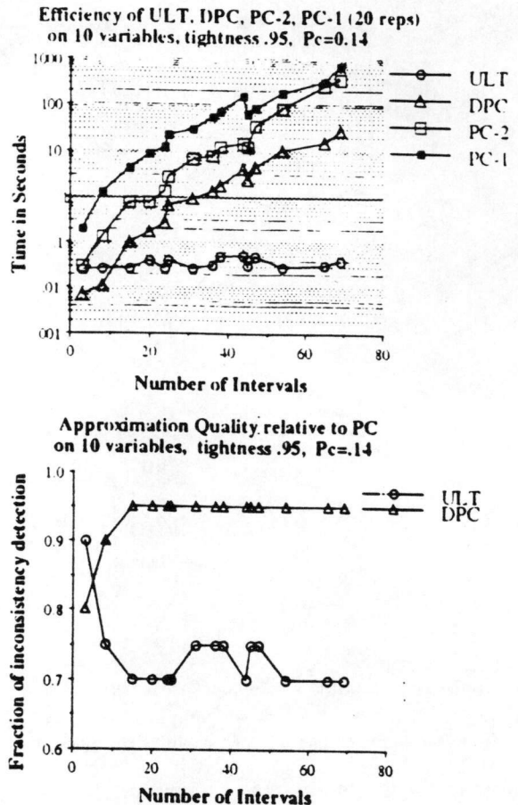
Figure 8: The execution time and quality of the approximation obtained by DPC and ULT to PC . Each point represents 20 runs on networks with 10 variables, .95 tightness, connectivity P_C = .14 and range [0, 600] .
