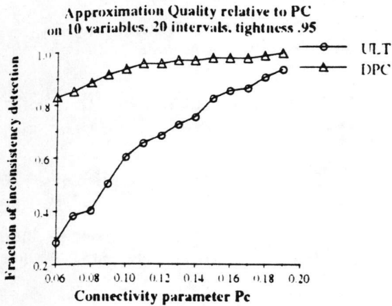
Figure 9: Quality of the approximation vs connectivity on problems with 10 variables, tightness .95 and range [0, 600]. We measured on problems of 3 intervals (top) where each point represents 1000 runs, and on 20 intervals (bottom) where each point represents 100 runs.
