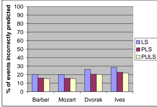
Figure 6: Incorrect predictions made by LS, PLS, and PULS
