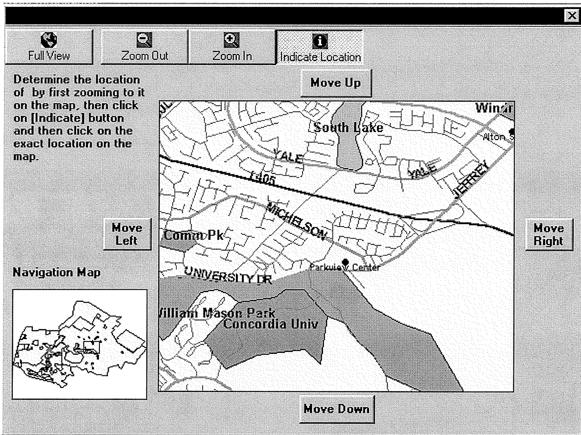
FIGURE 9 GIS Component
