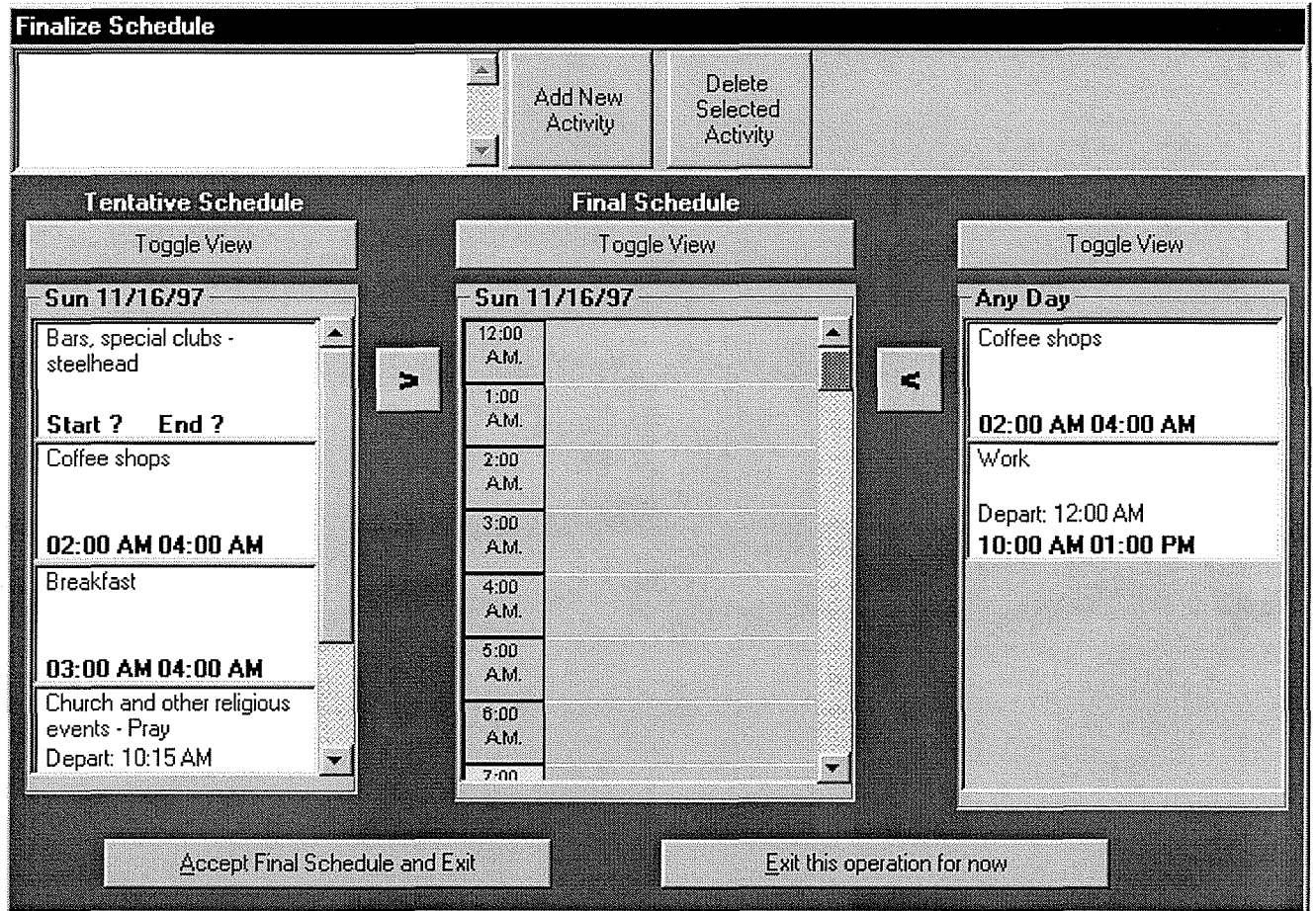
FIGURE 7 Finalize Schedule Interface
