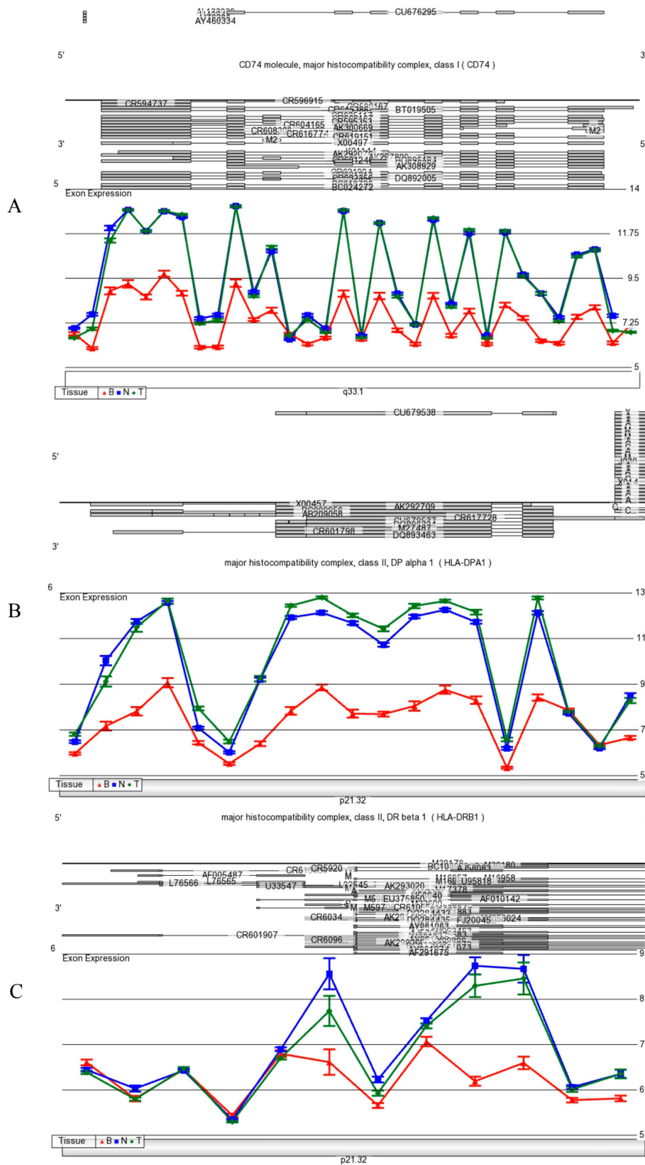
Figure 9. Exon microarray comparison of expression across brain samples (B), non-transformed whole blood samples and PBMC (N), and LCL EBV-transformed cell lines (T) for CD74 (Figure A); HLA-DPA1 (Figure B); and HLA-DRB1 (Figure C). In all three cases, the N and T levels (blood and immune cell levels) were higher than brain expression levels, and the higher expression levels by exon array were also confirmed by qPCR. The x-axis for each figure shows the probeset locations, and y-axis for each figure shows the probeset intensity in log 2 scale.
