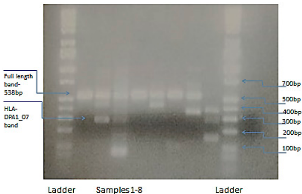
Figure 6. The gel images showed the multiple bands of HLA-DPA1 exon 2–4 from anterior cingulate brain samples. Full-length bands 538 bp and multiple bands of HLA-DPA1 exon 2–4 alternative splicing.
