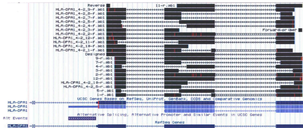
Figure 8. Alternative splicing of HLA-DPA1 in anterior cingulate cortex samples showing alignment of representative amplicons to RefSeq mRNA in UCSC Genome Browser. Forward and reverse sequences are aligned to RefSeq Genes using UCSC BLAT. The forward and reverse sequences are denoted with ‘f’ and ‘r’ in label, e.g., HLA-DPA1_4_2_9_f.ab1 is the same subject as 9-r.ab1.
