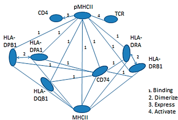
Figure 1. The interactions and molecular functions of three MHC Class II genes within the immune system involves antigen processing and presentation.
