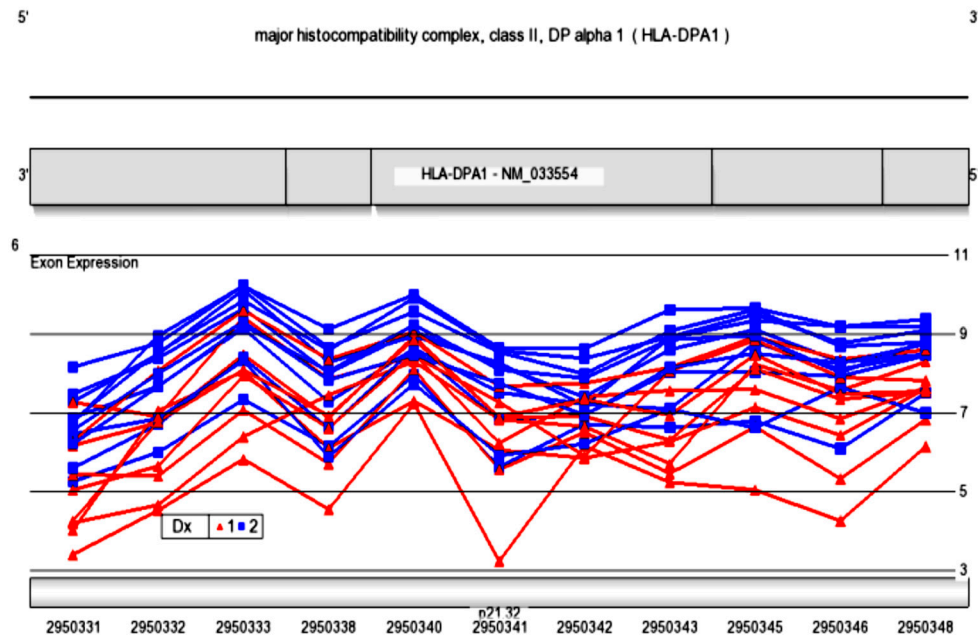
Figure 3. Individual samples for each probeset on HLA-DPA1 suggests differences within subjects consistent with a significant diagnosis by probeset interaction ( p = 1.6 \times 10^{-6} ).
