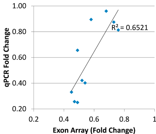
Figure 7. Comparison of fold change results for qPCR ( y -axis) and Affymetrix exon array ( x -axis) based upon genes shown in Table 10.
