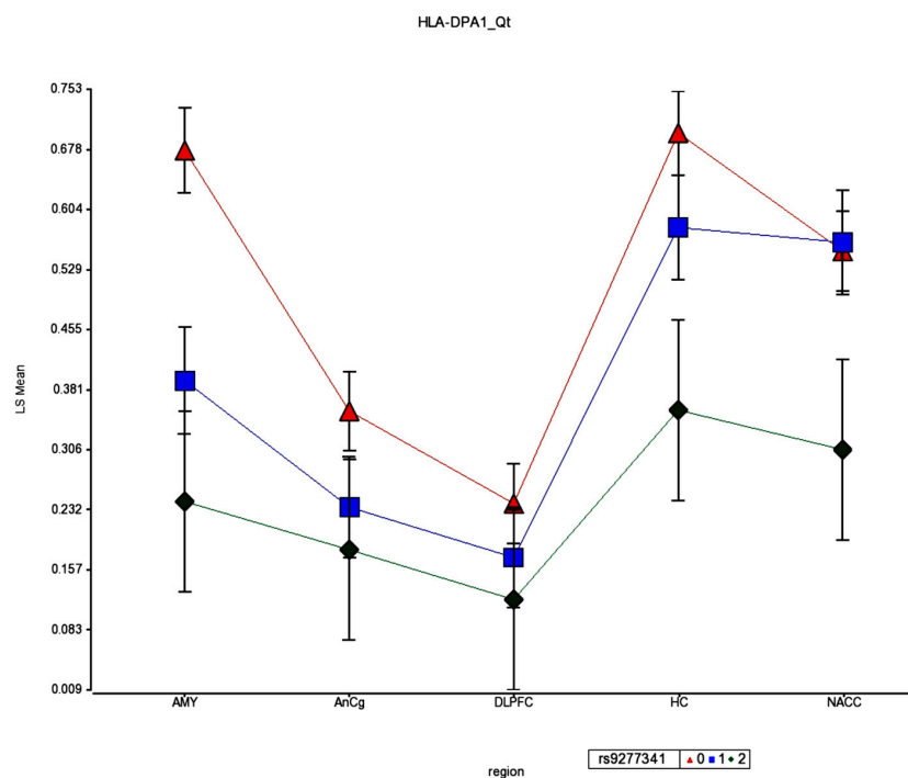
Figure 5. Genotype association analysis of HLA-DPA1 expression with rs9277341. The 0, 1, 2 groups represent the major allele, heterozygotes, and minor allele of SNP rs9277341. For the rs9277341, the SNP was sequenced and confirmed as (AA = 0), (AG = 1), and (GG = 2) on the negative strand. This corresponds with major and minor alleles, T (major) and C (minor) on the positive strand. The rs9277341 genotype main effect was significant for HLA-DPA1 expression ( p = 0.0002 ) across regions, the effect of region \times SNP rs9277341 was not significant, and region effect was highly significant ( 3.1 \times 10^{-17} ).
