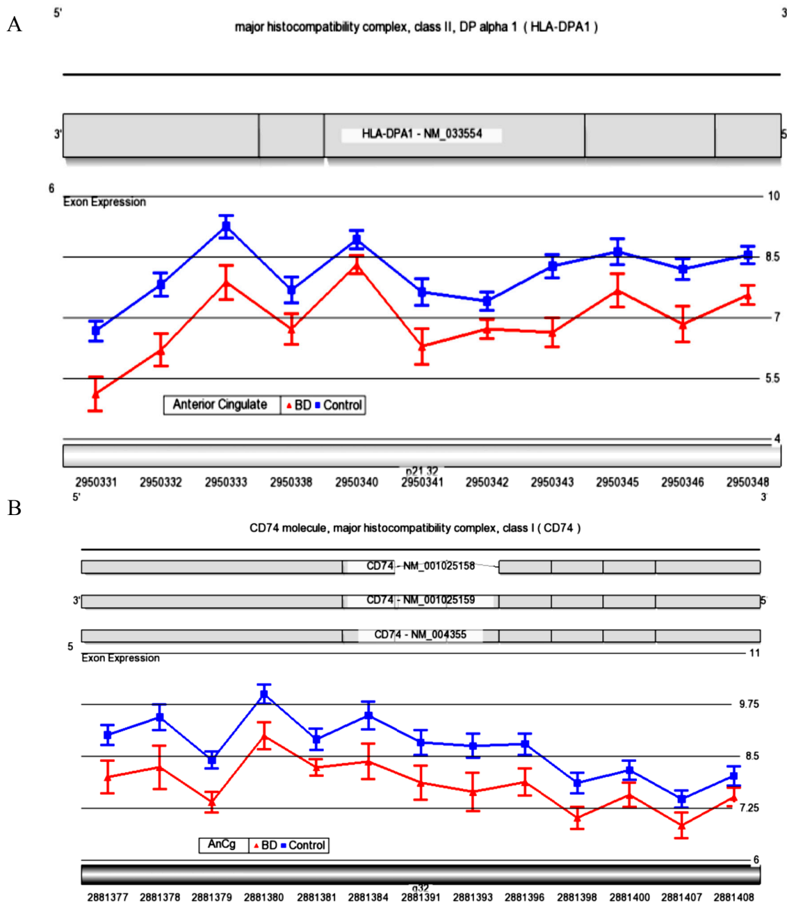
Figure 2. (A) HLA-DPA1 probeset shown on x -axis and probe intensity shown on y -axis in \log_2 scale. All probesets were significantly decreased ( p < 0.05 ) in bipolar disorder (BD, red) compared to controls (C, blue), except two probesets (2950338 and 2950345) that were at trend level ( p < 0.1 ). The p -values are shown in Table 4 for each probeset comparison; (B) The plot of CD74 for BD and C supports decreased expression along entire transcript.
