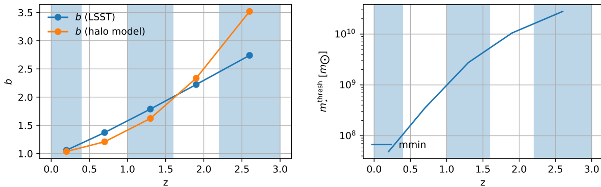
FIG. 2: Left: redshift binning and bias as a function of z for the LSST forecast. Right: HOD stellar mass threshold m_*^{\text{thresh}} as a function of z matched so that the galaxy number predicted by the halo model matches Eq. (8), extracted from the LSST science book.
