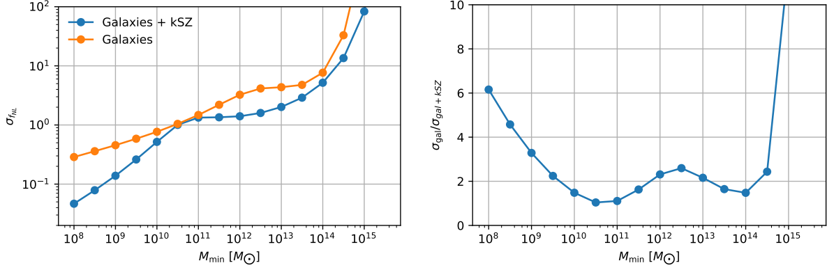
FIG. 7: Left: Constraints \sigma_{f_{NL}} for galaxies and for galaxies+kSZ as a function of M_{\min}^{\text{halo}} in a multi-tracer analysis. From left to right on the x-axis, each new dot removes one low mass bin from the forecast. For this analysis we used a survey with survey volume 100\text{Gpc}^3 and central redshift z_x = 1 . This forecast uses the halo model number densities n_h , biases b_h and power spectra P_{gg}, P_{ge} . Right: Improvement factor due to adding the kSZ information.
