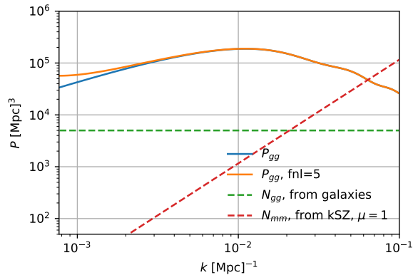
FIG. 1: Galaxy power spectra and noise power spectra for an experimental configuration corresponding to the DESI experiment (with galaxy density and CMB noise according to our baseline 1 defined in Table I). At large scales, where the f_{NL} signal is strongest, we get a much lower noise using kSZ tomography than with galaxies alone, due to the k^2 scaling of the kSZ reconstruction noise. The chosen f_{NL} value of 5 is near the 1\sigma sensitivity for this configuration. All power spectra are shown at z = 1 and for |\mu| = 1 (radial modes), and the galaxy power spectra include the RSD term.
