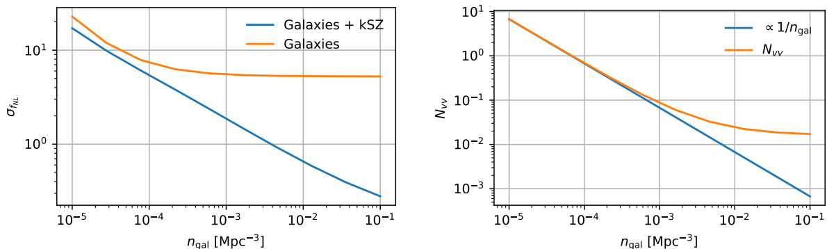
FIG. 4: Left: Sensitivity \sigma_{f_{NL}} as a function of galaxy density n_{\text{gal}} for baseline 2. Galaxy density is a critical parameter for our method, in particular because increasing it improves the shot noise of the galaxy mode for sample variance cancellation. For clarity in this plot we have kept the bias constant, however of course highly biased galaxies are limited in number. Right: Velocity reconstruction noise N_{vv} as a function of galaxy density n_{\text{gal}} for baseline 2. This illustrates that for baseline 2 the galaxy density is so large that with CMB S4 noise levels we are close to signal-to-noise saturation of the velocity reconstruction as a function of n_{\text{gal}} .
