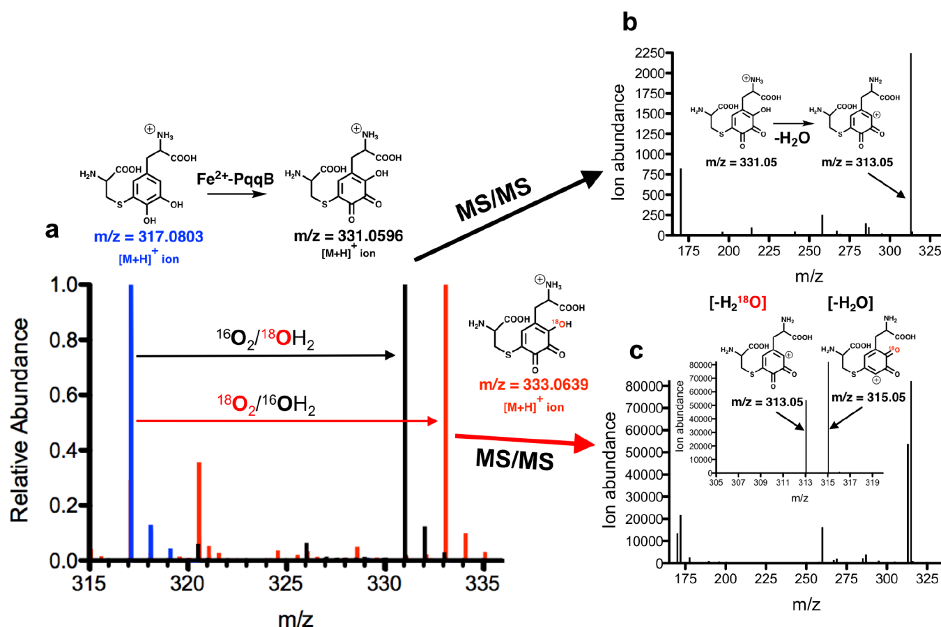
Figure 4. High-Resolution Mass Spectrometric (HRMS) analyses of \text{Fe}^{2+} -dependent PqqB hydroxylation.
