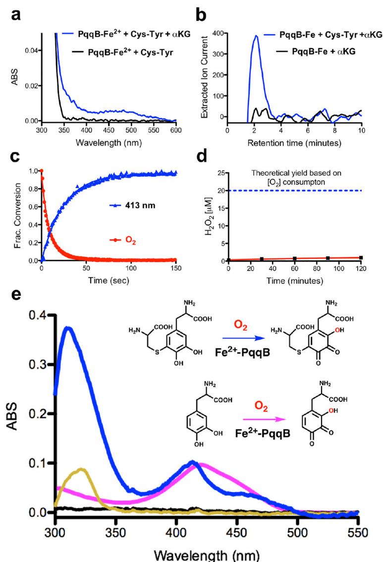
Figure 3. Reaction details of \text{Fe}^{2+} -dependent PqqB hydroxylation.
