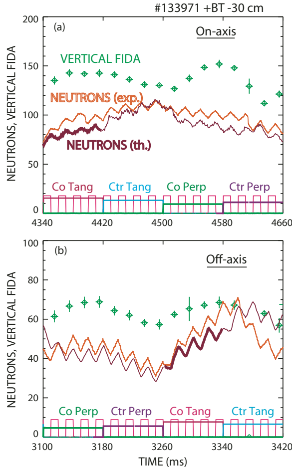
Figure 15. Time evolution of the neutron rate and of the R = 180 cm vertical FIDA channel during the (a) on-axis and (b) off-axis phase of an H-mode discharge. The 330L co-tangential beam viewed by the vertical FIDA diagnostic injects continuously at 50% duty cycle, while the steady source cycles through the four different angles of injection. The neutron rate predicted by TRANSP is most reliable during the phase marked by the thick line because toroidal rotation data is available then; the absolute calibration is adjusted 20% to facilitate comparison of the time evolution. The FIDA data are conditionally averaged over several cycles of beam injection. I_p = 0.9 MA; B_T = +2.1 T; z_0 = -30 cm during the off-axis phase; off-axis profiles shown in figure 8.
