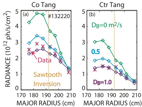
Figure 25. Vertical FIDA profile (x) near the end of co-tangential (a) and counter-tangential (b) injection in a full-size, on-axis, discharge. After conditional averaging, the random errors are smaller than the symbols in this steady-state L-mode discharge. The solid lines are the predicted profiles for ad hoc diffusion of D_B = 0, 0.5 and 1.0\text{ m}^2\text{ s}^{-1} . The vertical dashed line indicates the sawtooth inversion radius inferred from ECE data. B_T = -2.0 T; I_p = 0.6 MA; \bar{n}_e = 1.9 \times 10^{19}\text{ m}^{-3} ; T_i(0) = 2.9 keV; T_e(0) = 3.4 keV.
