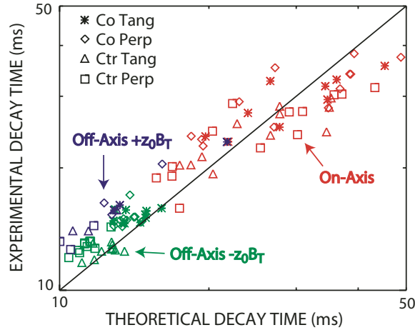
Figure 11. Experimental decay time versus decay time predicted by TRANSP for many different discharges. The angle of beam injection is represented by the symbols and the colors indicate on-axis injection, off-axis with z_0 B_T > 0 and z_0 B_T < 0 . The solid line shows agreement between theory and experiment.
