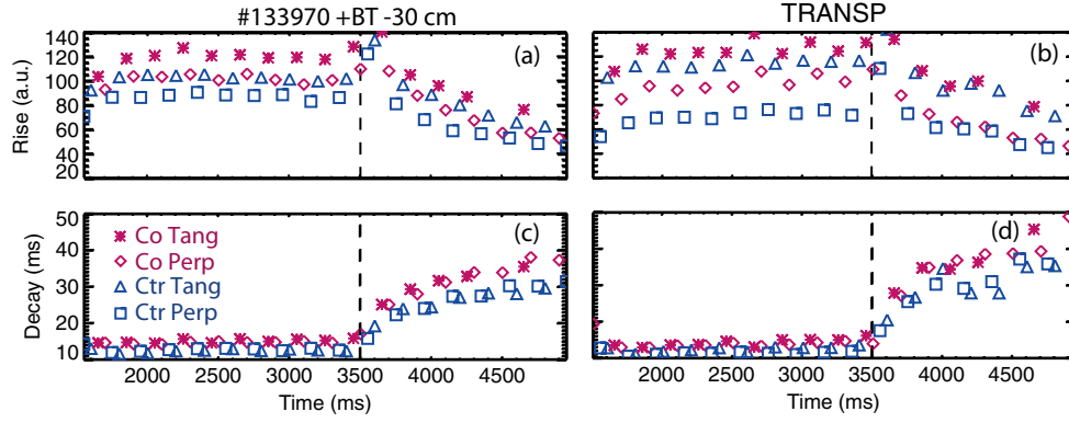
Figure 9. Experimental and theoretical rates of rise (a), (b) and decay times (c), (d) for a small plasma with +B_T . The magnetic axis is at z_0 = -30 cm until 3500 ms and reaches the midplane \sim 70 ms later. The angle of beam injection is represented by the symbols.
