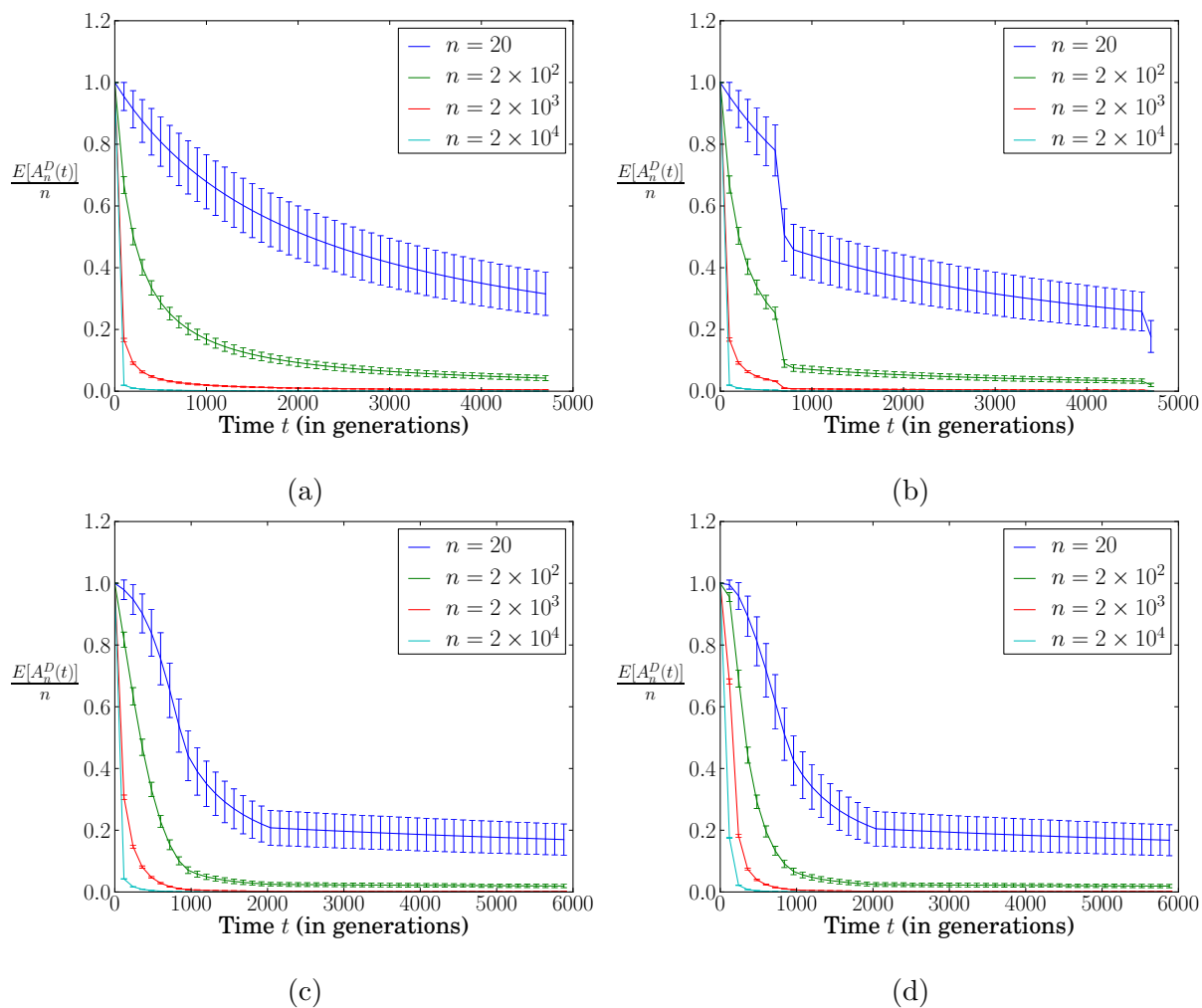
Figure 4.7: The expectation (solid line) and standard deviation (vertical whiskers) of the NLFT under the DTWF model. (a) MODEL 1. (b) MODEL 2. (c) MODEL 3. (d) MODEL 4.
