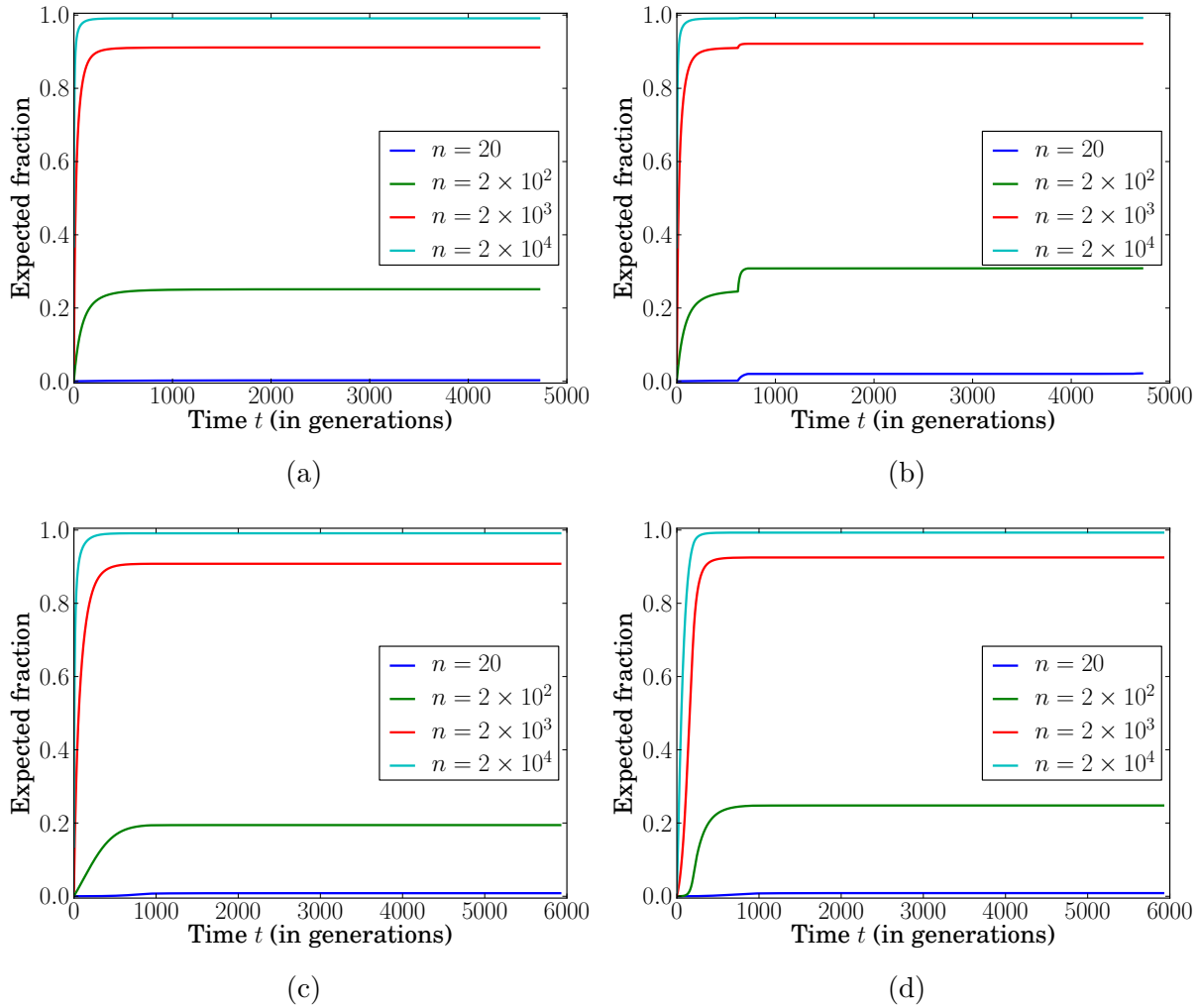
Figure 4.3: Expected proportion of lineages (relative to n - 1 , where n is the sample size at present) that are lost in generations when more than one lineage is lost, from the present up to time t in the past. For each generation t on the x -axis, the y -axis is the expected number of lineages that have been lost due to coalescence events in those generations from 0 to t where more than one lineage is lost, normalized by the quantity n - 1 , which is the total number of lineages that are lost over all generations. The plots correspond to (a) MODEL 1, (b) MODEL 2, (c) MODEL 3, and (d) MODEL 4. The sharp jumps in the plot for MODEL 2((b)) corresponds to the beginning (backwards in time) of population bottlenecks when the population size declines substantially, thus instantaneously increasing the rate at which lineages find common ancestors and are lost. For small sample sizes relative to the population size ( n = 20 and n = 200 ), it is unlikely for more than one lineage to be lost in a single generation. In contrast, for large sample sizes ( n = 2 \times 10^4 ), almost all the lineages are lost in generations when more than one lineage is lost.
