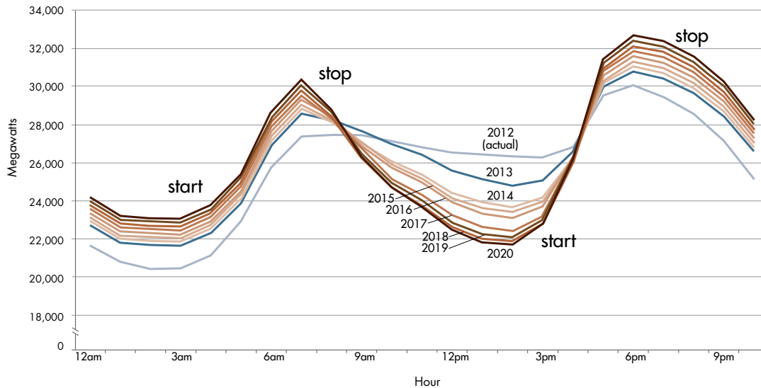
Figure 3.2. This “duck curve” shows net demand (total energy demand minus renewable energy generation) over time on a specific day, January 11. The duck curve illustrates the steep ramps necessary when other sources of energy generation must be quickly shut down or brought online to either make room or compensate for renewable energy generation. Licensed with permission from the California ISO.
