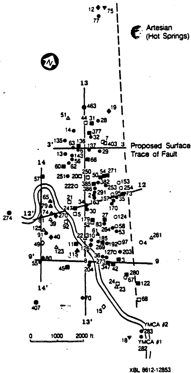
Figure 2. Wells supplying temperature data. Lines drawn across the wells indicate the location of temperature profile cross-sections.
