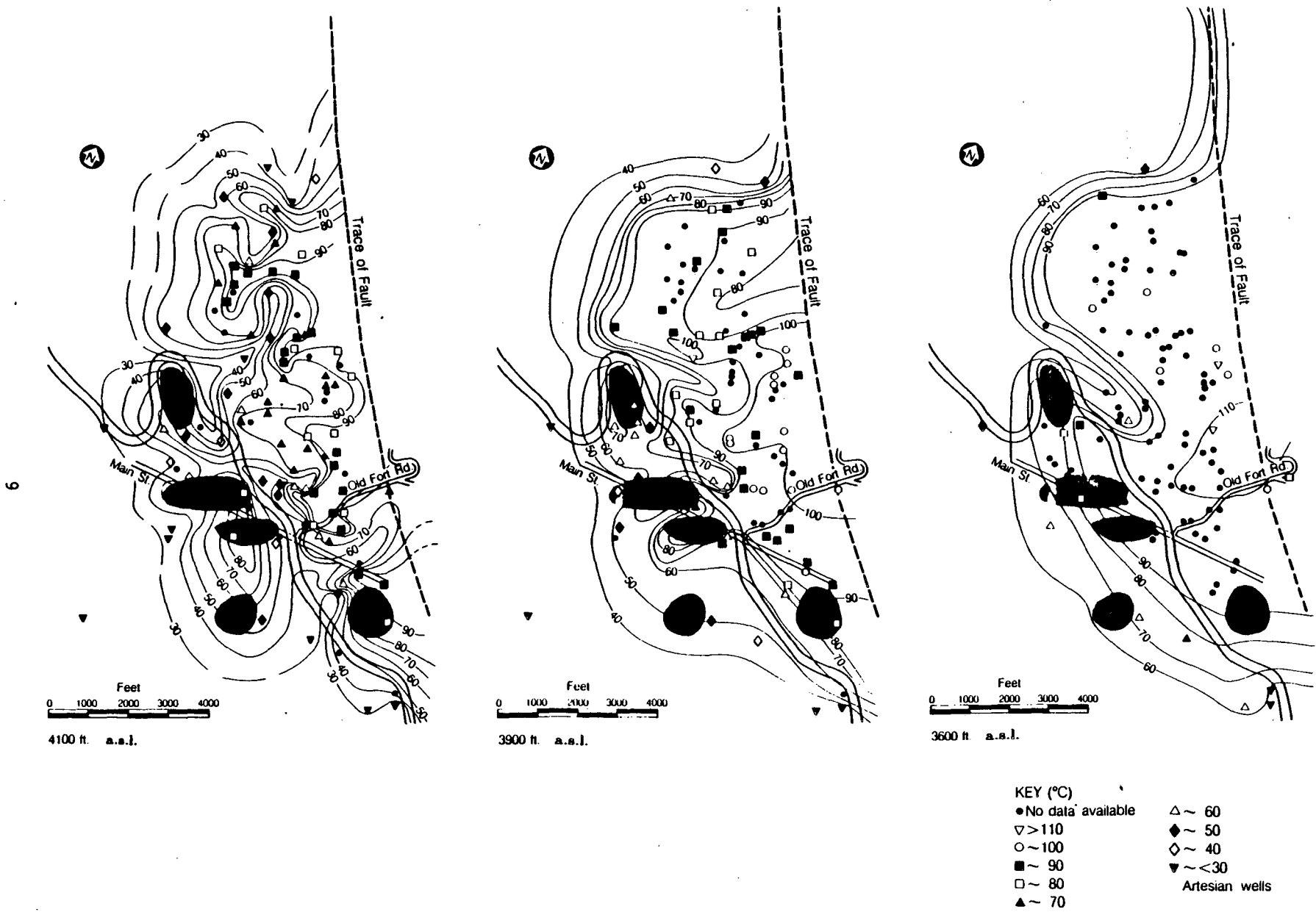
Temperature contour maps drawn at 4100 ft, 3900 ft and 3600 ft.
