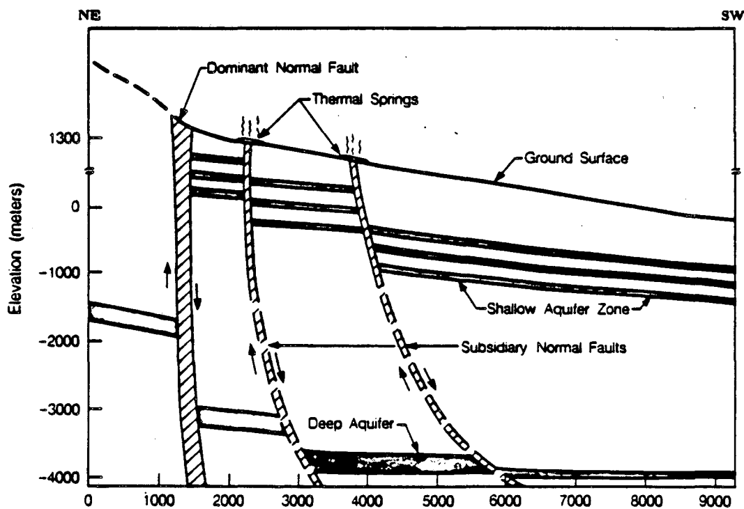
Figure 8. Conceptual model for the Klamath Falls geothermal system.
