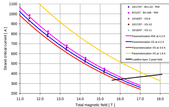
Figure 2: Critical current (A) vs. applied field (T) measurements and parameterization curves of virgin
