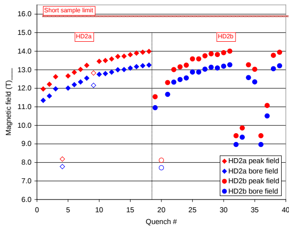
Figure 10: Training quenches of HD2a and HD2b.
