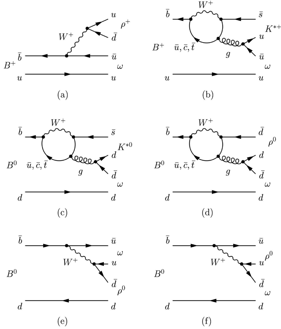
FIG. 1. Representative Feynman diagrams for B \rightarrow \omega \rho and B \rightarrow \omega K^* decays: (a) external tree; (b,c) CKM-favored gluonic penguins; (d) CKM-suppressed penguin; (e,f) destructively interfering color-suppressed trees.
