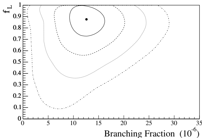
FIG. 4. Distribution of \chi^2 = -2 \ln \mathcal{L}(f_L, \mathcal{B}) for B^+ \rightarrow \omega \rho^+ . The solid dot gives the central value; curves give the contours in one-sigma steps ( \Delta\sqrt{\chi^2} = 1 ) out to four sigma.
