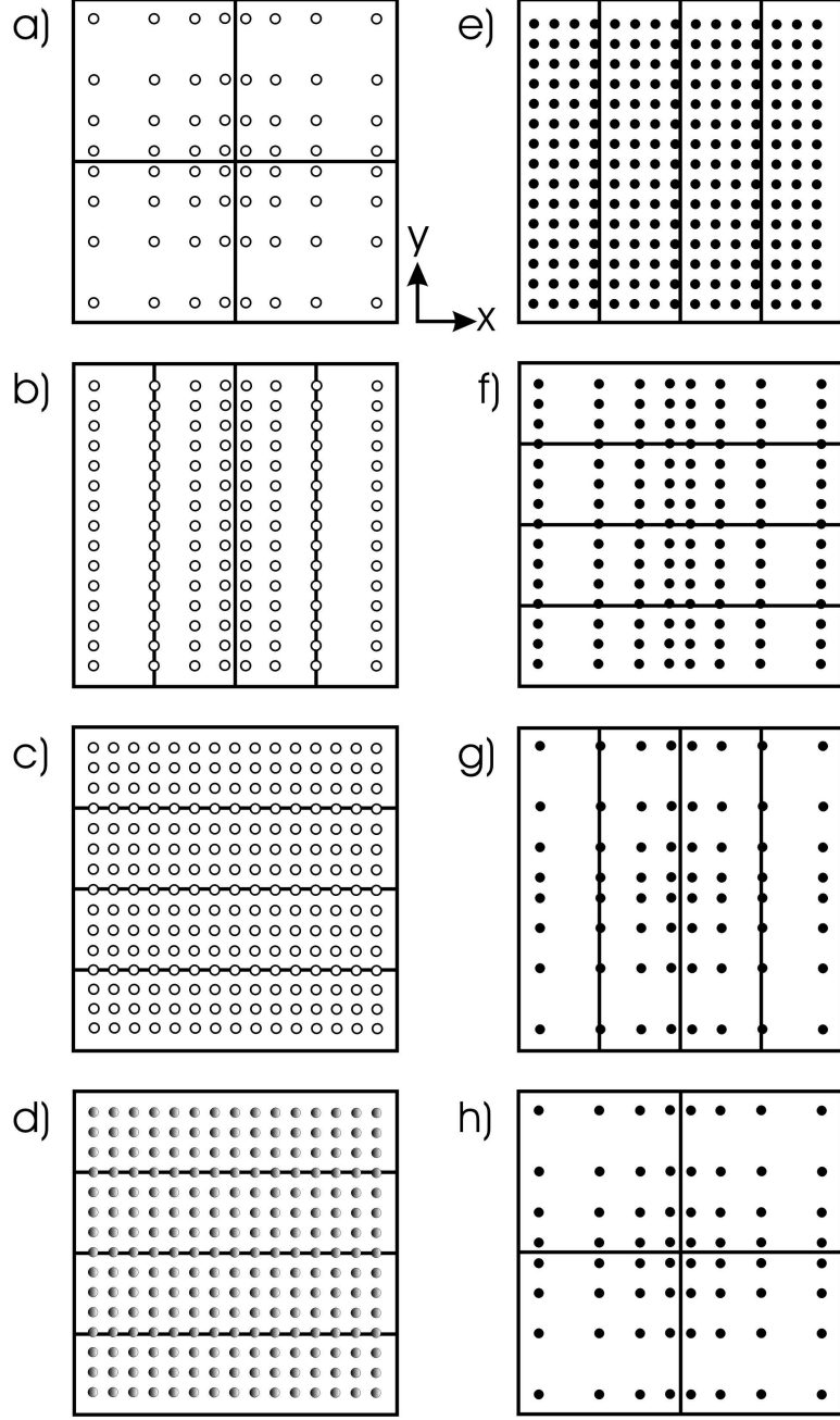
FIG. 2. Parallel field upward continuation scheme involving remapping, interpolation and both forward and inverse 2-D FFT along both horizontal dimensions x and y of the surface grid. (a) Initial distribution, (b) remap, y -interpolation, (c) remap, x -interpolation, (d) \text{FFT}(x) , (e) remap, \text{FFT}(y) , upward continuation, \text{FFT}^{-1}(y) , remap, \text{FFT}^{-1}(x) , (f) x -interpolation, (g) remap, y -interpolation, (h) remap to initial distribution.
