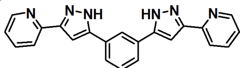
Scheme 1. Molecular structure of ligand L.
