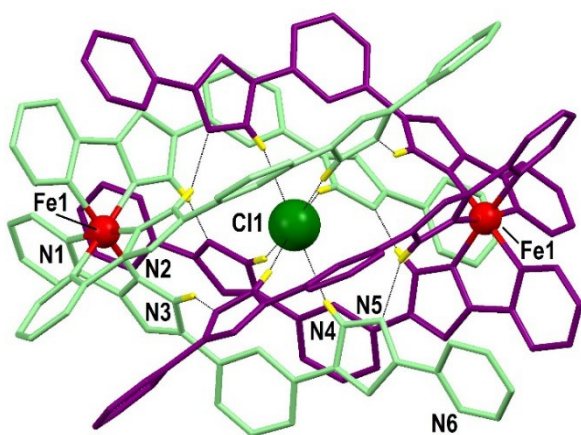
Figure 2. Representation of the (\text{X}@\text{[FeL}_3\text{]}_2)^{3+} supramolecular assembly in 1 ( \text{X}=\text{Cl}^- ). The ligands of each [\text{FeL}_3]^{2+} unit are in a different colour (green and purple, respectively). Unique heteroatoms are labelled. Only H atoms of N-H groups are shown (yellow). The same moiety is present in 2 to 5 .
