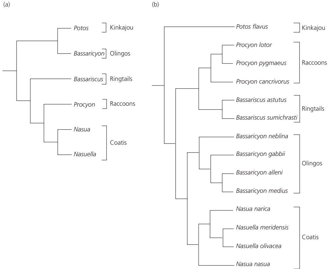
Figure 2.4 (a) Phylogenetic tree showing relationships among the genera of the Procyonidae based on morphological characters (Decker and Wozencraft 1991; Baskin 2004). Also see Ahrens (2012) for an alternative topology based on many more additional characters. (b) Consensus phylogenetic tree displaying the relationships among the 14 recognized species within the Procyonidae. The tree topology is based on a synthesis of the following studies: Fulton and Strobeck (2007); Koepfli et al. (2007); Helgen et al. (2009); Eizirik et al. (2010); and Helgen et al. (2013). The phylogenetic tree was generated using Mesquite (Maddison and Maddison 2016).
