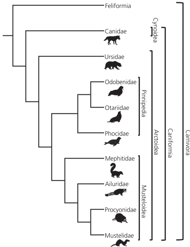
Figure 2.1 Phylogenetic tree depicting the relationships among the four families of the Musteloidea and the position of the Musteloidea within the Caniformia. Other major clades are also indicated. The tree topology is based on the studies of Sato et al. (2009), Eizirik et al. (2010) and Nyakatura and Bininda-Emonds (2012). The phylogenetic tree was generated using Mesquite (Maddison and Maddison 2016).
