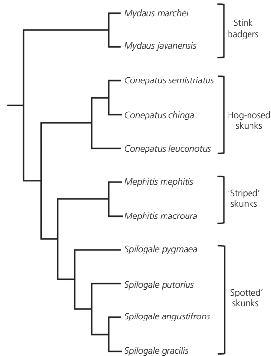
Figure 2.3 Consensus phylogenetic tree showing the relationships among all the extant species of the Mephitidae. The relationships among genera and species are based on a synthesis of the following molecular studies: Dragoo et al. (1993); Dragoo and Honeycutt (1997); Dragoo et al. (2003); Eizirik et al. (2010); Ferguson et al. (2017) and Schiaffini et al. (2013b). The phylogenetic tree was generated in Mesquite (Maddison and Maddison 2016).
