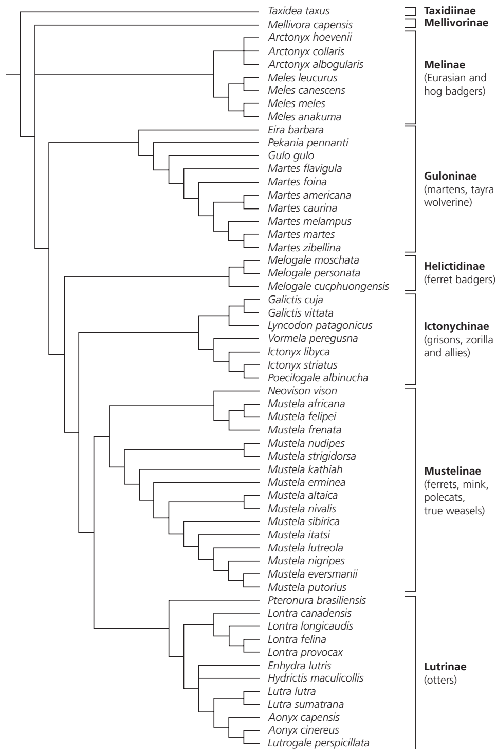
Figure 2.2 Phylogenetic tree showing the pattern of relationships among all extant genera and 57 of the 65 proposed, or recognized, species within the family Mustelidae. Bracketed clades or lineages define the eight recognized subfamilies. The following six species are not depicted in the tree due to absence of formal phylogenetic studies (but see Nyakatura and Bininda-Emonds 2012): Melogale everetti , Melogale orientalis (Melinae); Martes gwatkinsii (Guloninae); Mustela lutreolina , Mustela subpalmata (Mustelinae); and Aonyx congicus (Lutrinae). The tree shown is a consensus tree assembled from the following studies: Koepfli and Wayne. (2003); Koepfli et al. (2008a, b); Sato et al. (2009); Harding and Smith (2009); Del Cerro et al. (2010); Nadler et al. (2011); Yu et al. (2011b); Sato et al. (2012); Dawson and Cook (2012); B. Li et al. (2014); and Malyarchuk et al. (2015). The phylogenetic tree was generated in Mesquite (Maddison and Maddison 2016).
