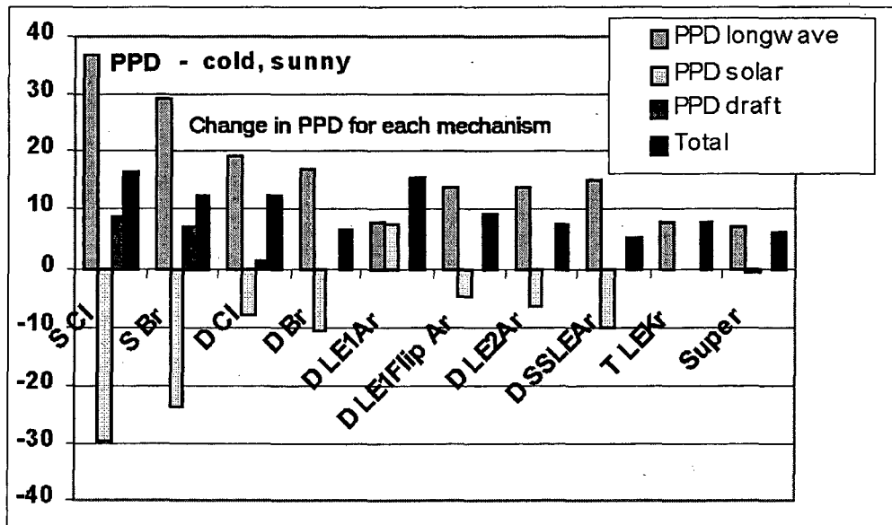
Figure 4. Long-wave, solar radiation and draft contributions to the Percentage People Dissatisfied for a large glazed door.
