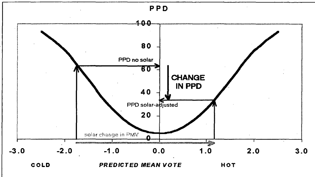
Figure 2. Fanger PPD-PMV relationship, showing adjustment for solar load.
