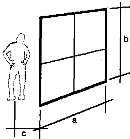
Figure 3. Occupant/window geometry used for view factor calculations.
