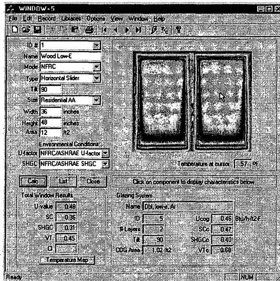
Figure 9. Concept for mapping of glazing inside surface temperature in WINDOW+5 computer program (LBNL, 1999).
