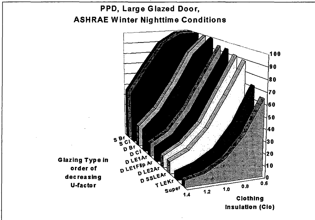
Figure 7. Percentage People Dissatisfied under ASHRAE Winter Conditions (No. 8 in Table 2) as a function of clothing level and glazing U-factor.
