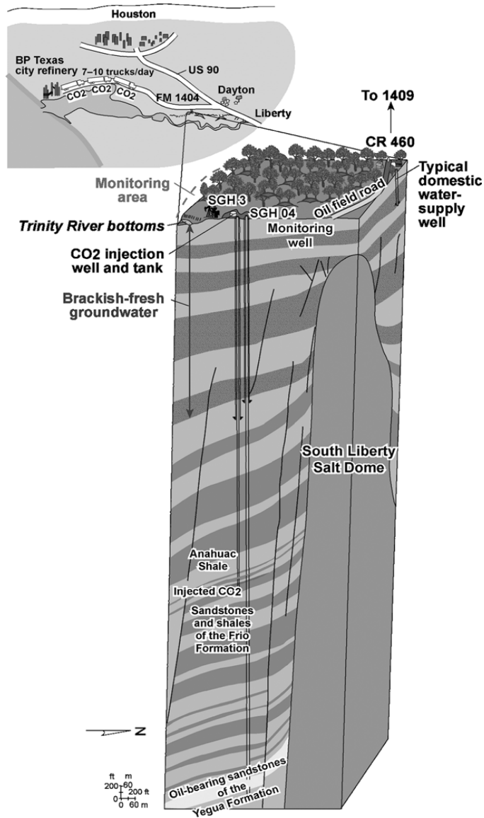
Figure 1. Location of the Frio Brine Pilot field site, 60 km from Houston, Texas, and a schematic of the underlying stratigraphy. CO 2 was injected in the Frio Formation, capped by the low-permeability Anahuac Shale. (Courtesy S. Hovorka)
