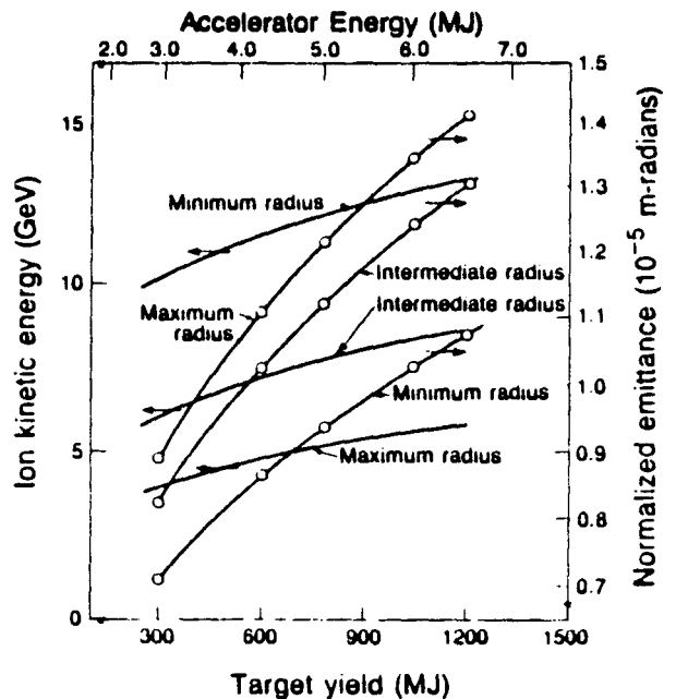
For a Given Target Yield, the Required Accelerator Output is Defined for a Given Ion Mass
