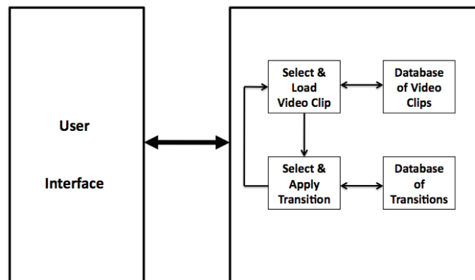
Figure 3: Generative Engine
