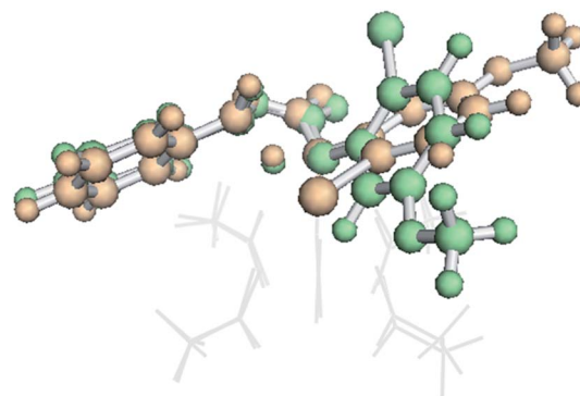
Fig. 6 Conformational dependence of IRC behaviour. An overlay of two conformations of β-TS 1 for formation of the trans product for the substrates in entries 1 and 2 in the table inset in Fig. 5. 54 The lowest energy conformation (orange, IRC leading to the fragmented product) and the higher energy conformation (green, IRC leading to the β-lactone product) differ only by rotation of the substituted phenyl ring. The Rh 2 (OAc) 4 catalyst is represented as gray lines for clarity. Both structures were optimized at the B3LYP/6-31G(d), LANL2DZ level of theory.
