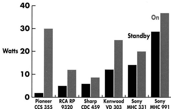
Figure 1. Full and standby power draws of some compact audio systems.
