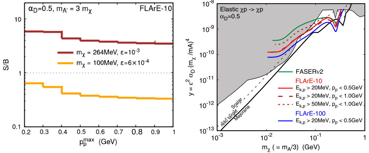
FIG. 2. Left: the signal-to-background ratio S/B for the elastic scattering signature for FLArE-10 and the two DM benchmark scenarios indicated as a function of the maximum momentum of the outgoing proton p_p^{\max} . The expected number of neutrino-induced background events for selected values of p_p^{\max} can be found in Table II, and we assume the detectability threshold of E_{k,p} > 20 MeV for the proton kinetic energy. Right: the projected 90% C.L. exclusion bounds for the elastic scattering signature for FASER \nu 2 with 300 \text{ MeV} \lesssim p_p \lesssim 1 \text{ GeV} (green), FLArE-10 (red), and FLArE-100 (blue) with the proton energy and momentum cuts indicated. Current bounds exclude the gray-shaded region; see Sec. VII for details. The thermal relic targets for the Majorana fermion DM and complex scalar DM models are also shown.
