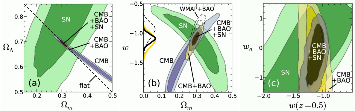
Figure 1.2: Constraints on the present matter fraction \Omega_m and dark energy model parameters. Dark and light shaded regions indicate 68.3% and 95.4% confidence levels, respectively. “CMB” is Planck+WP, “BAO” is the combination of SDSS-II, BOSS, and 6dFGS, and “SN” is Union2. (a) The present dark energy fraction \Omega_\Lambda vs. \Omega_m , assuming a \Lambda CDM model. CMB data, especially when combined with BAO constraints, strongly favor a flat universe (diagonal dashed line). (b) The dark energy equation of state w vs. \Omega_m , assuming a constant value of w . The dashed contours show the 68.3% and 95.4% CL regions for the combination of WMAP9 and BAO data. Curves on the left vertical axis show the probability distributions for w (normalized arbitrarily), after marginalizing over \Omega_m , for the CMB+BAO and CMB+BAO+SN combinations (yellow and black, respectively), using Planck+WP CMB data, and for the WMAP9+BAO combination (dashed black). (c) Constraints on the two parameters of the dark energy model with a time-dependent equation of state given by Eq. (1.4): w(z = 0.5) and w_a = -dw/da .
