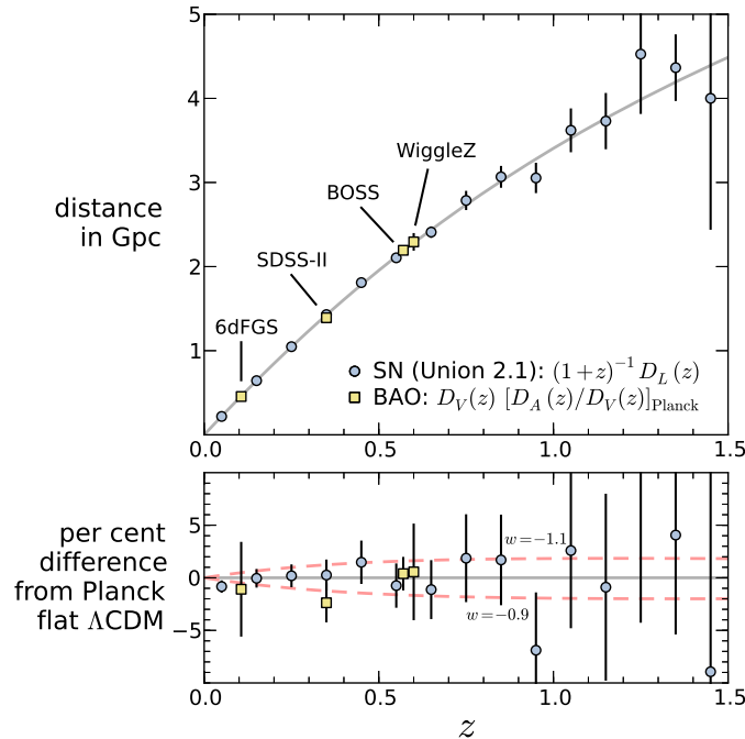
Figure 1.1: The distance-redshift relation measured from Type Ia SNe and BAO compared to the predictions (gray curve) of a flat \Lambda CDM model with the best-fit parameters inferred from Planck+WP CMB data. Circles show binned luminosity distances from the Union2.1 SN sample, multiplied by (1+z)^{-1} to convert to comoving angular diameter distance. Squares show BAO distance measurements, converted to D_{A,c}(z) for the Planck+WP cosmology and sound horizon, from the references given in the text. The lower panel plots residuals from the Planck+WP \Lambda CDM prediction, with dashed curves that show the effect of changing w by \pm 0.1 while all other parameters are held fixed. Note that the SN data points can be shifted up or down by a constant factor to account for freedom in the peak luminosity, while the BAO points are calibrated to 0.4% precision by the sound horizon scale computed from Planck+WP data.
