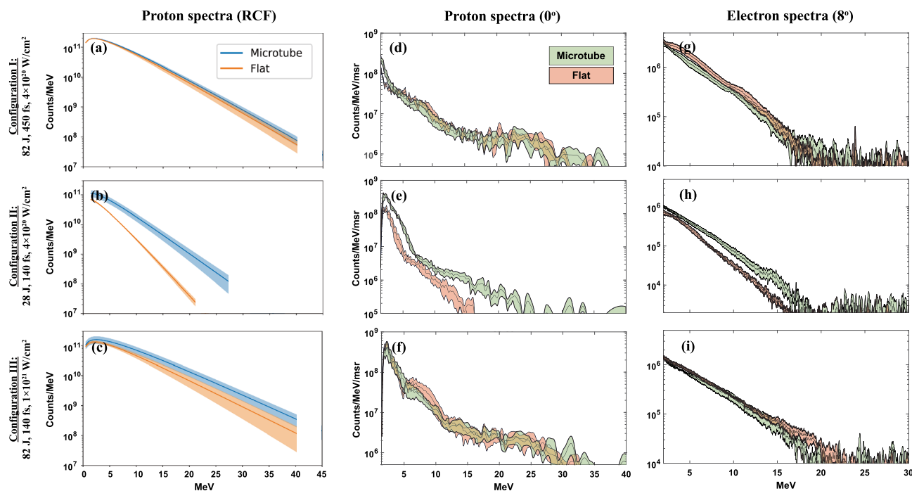
Figure 2. Proton and electron spectra for each laser configuration. (a–c) Maxwell–Boltzmann fits to the RCF spectra, with good correspondence to the Thomson parabola at 0° (d–f). The full energy configurations (top and bottom rows) show a minimal difference between proton spectra from flat and microtube targets. The middle row, however, indicates that for the 28 J configuration, microtubes enhance maximum proton energy by 50%, and total proton yield by 3× (b,e). A corresponding enhancement in electron spectra, namely a 12% temperature increase, is also observed in (h). The width of each spectrum represents the error bands, as averaged over ~ 3–5 shots for RCF, and ~ 10 shots for the TP and EPPS. Key takeaways from the spectra are summarized in Table 2.
