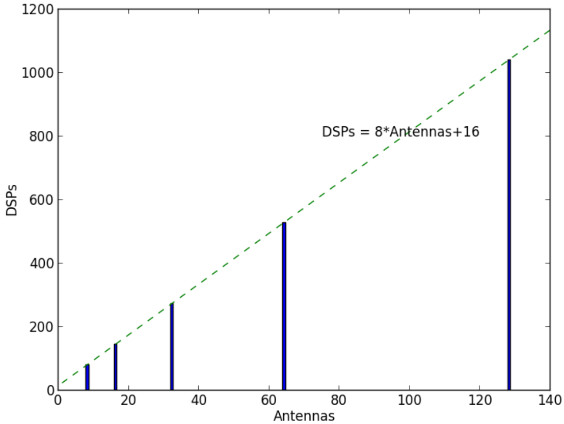
Figure 5.4: Cross-Correlator X-engine DSP Utilization
