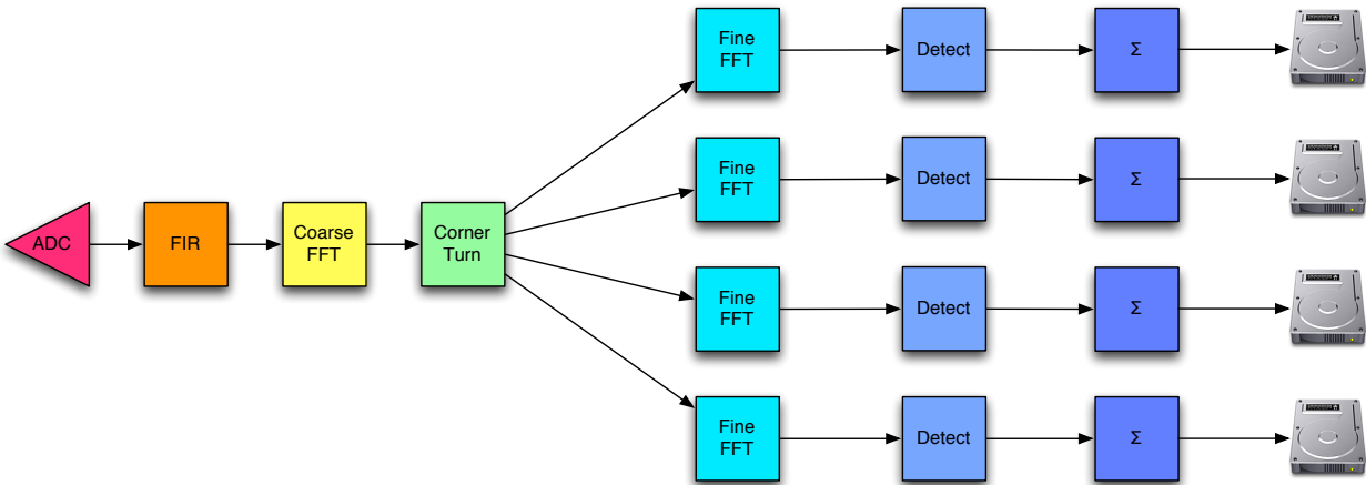
Figure 6.2: Example High Resolution Spectrometer Dataflow Model
