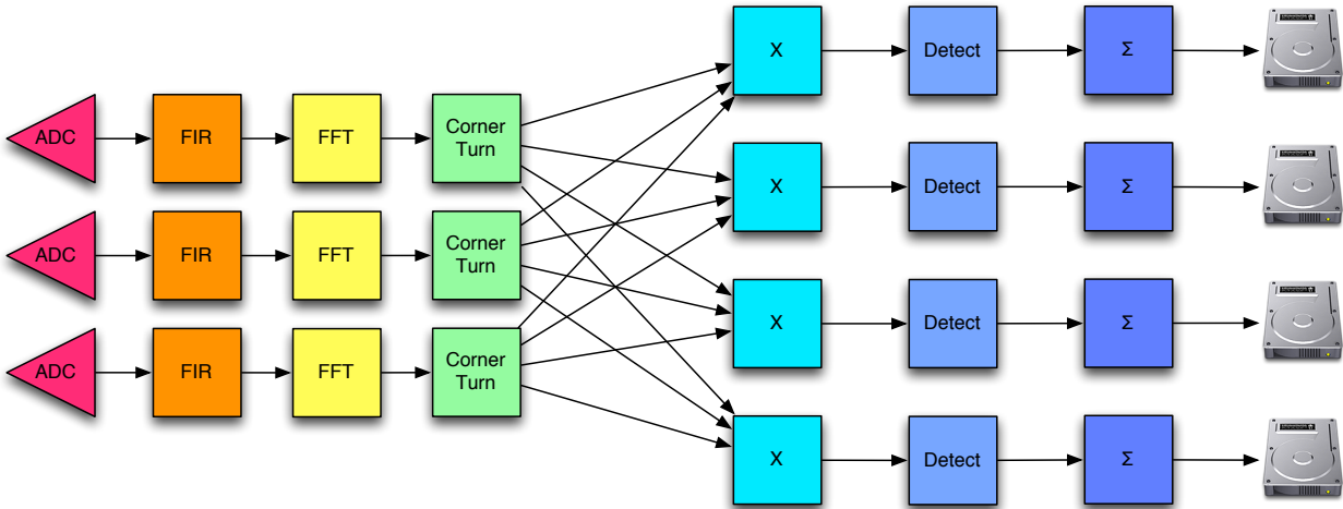
Figure 6.6: Example FX Correlator Dataflow Model
