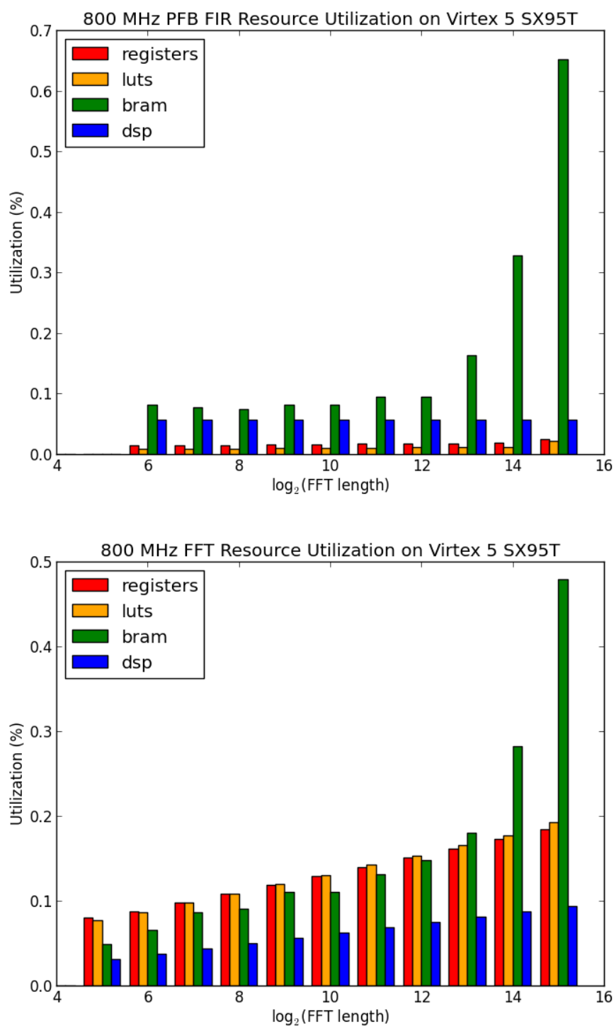
Figure 5.2: PFB FIR and FFT benchmark data on the Virtex 5 SX95T
