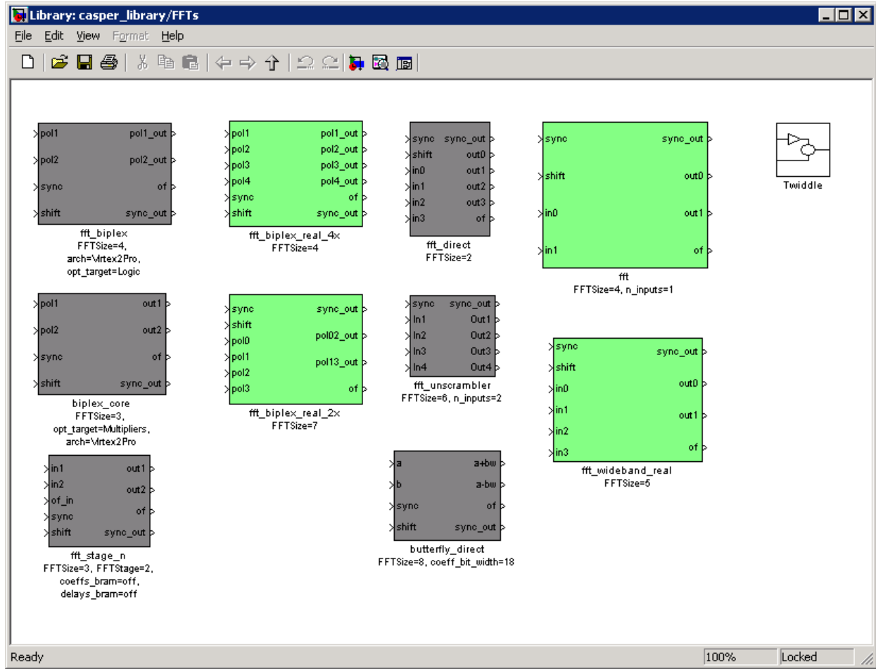
Figure 3.6: CASPER FFT Library
