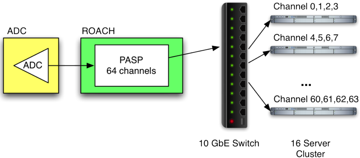
Figure 3.17: Example high level spectrometer architecture
