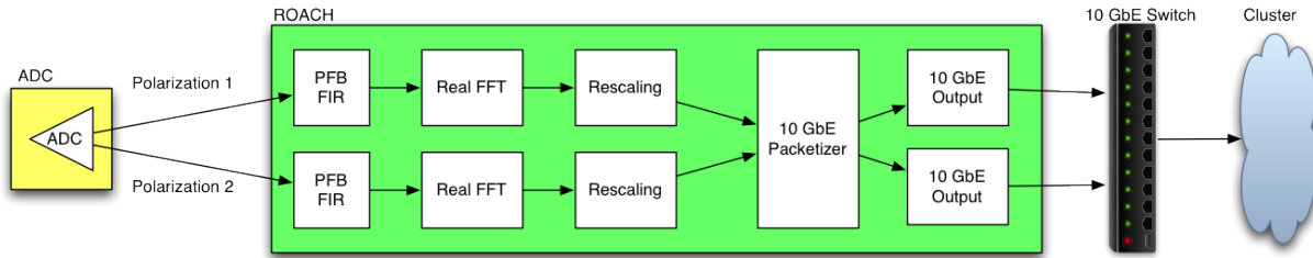
Figure 3.13: PASP Dataflow (reprinted from Filiba and Werthimer [8])
