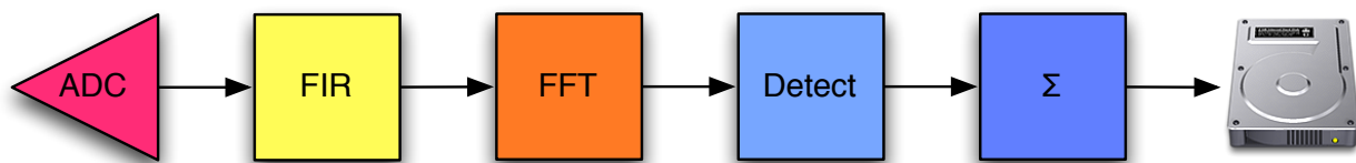
Figure 6.1: General Spectrometer Dataflow Model
