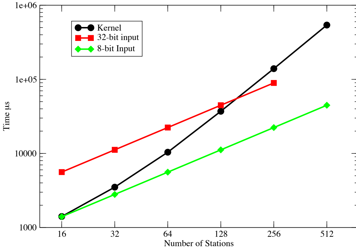
Figure 3.1: xGPU Performance as a function of array size (reprinted from Clark, La Plante, and Greenhill [3])
