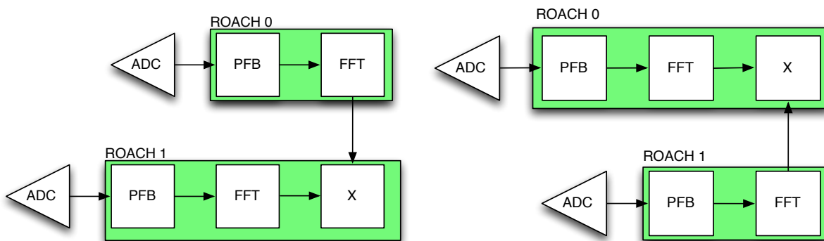
Figure 5.5: Example of Design Symmetry in the ILP
