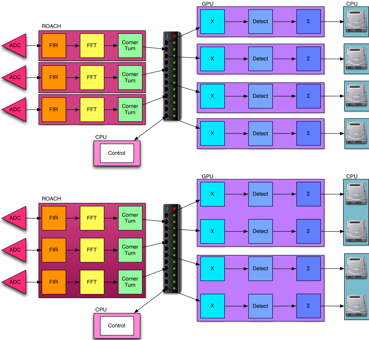
Figure 4.6: Two potential mappings for the FX Correlator
