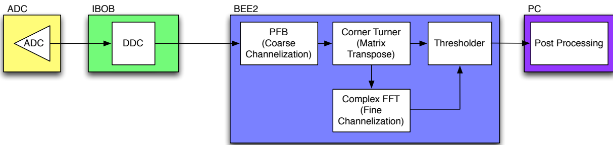
Figure 3.10: SERENDIP V.v Block Diagram
