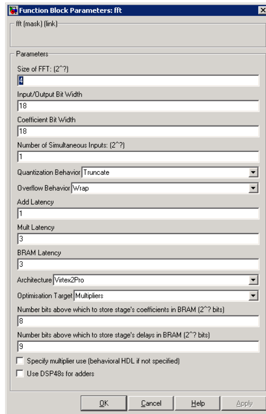
Figure 3.7: CASPER FFT Options Menu
