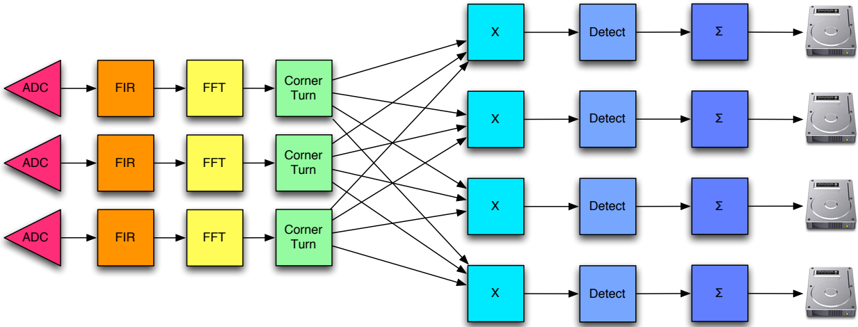
Figure 4.3: Example FX Correlator Dataflow Model Demonstrating Blocktypes
