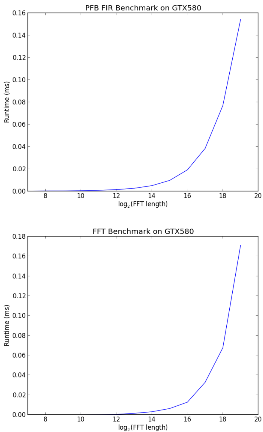
Figure 5.3: PFB FIR and FFT benchmark data on the GTX 580
