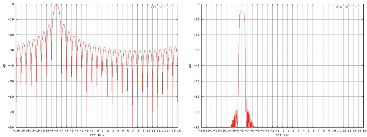
Figure 3.8: A comparison of FFT and PFB response
