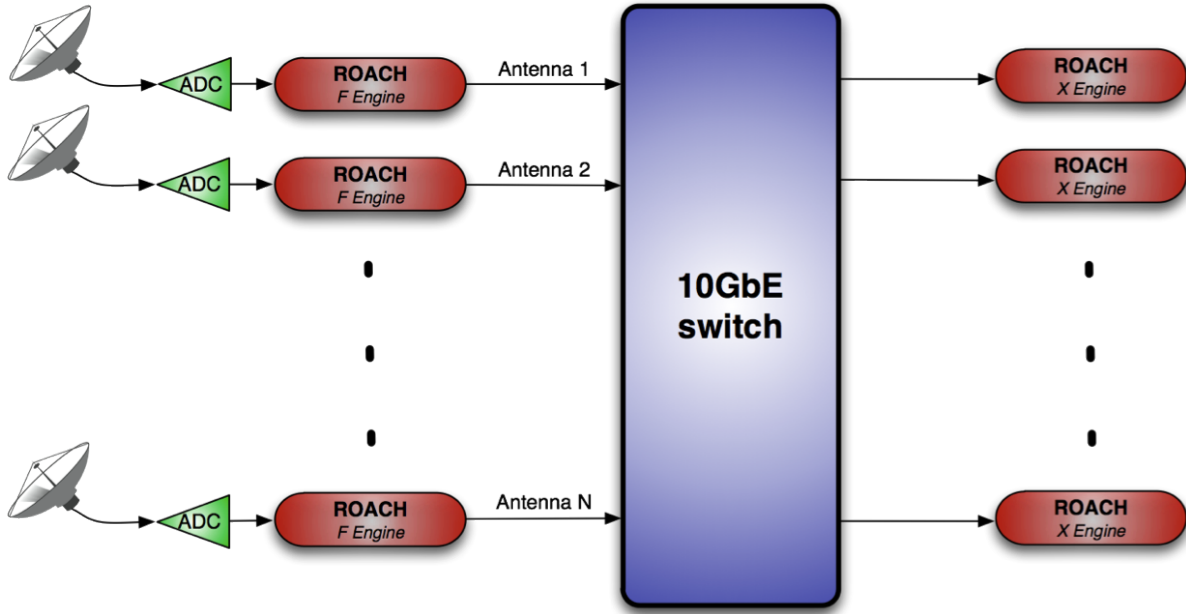
Figure 3.12: CASPER Correlator Architecture
