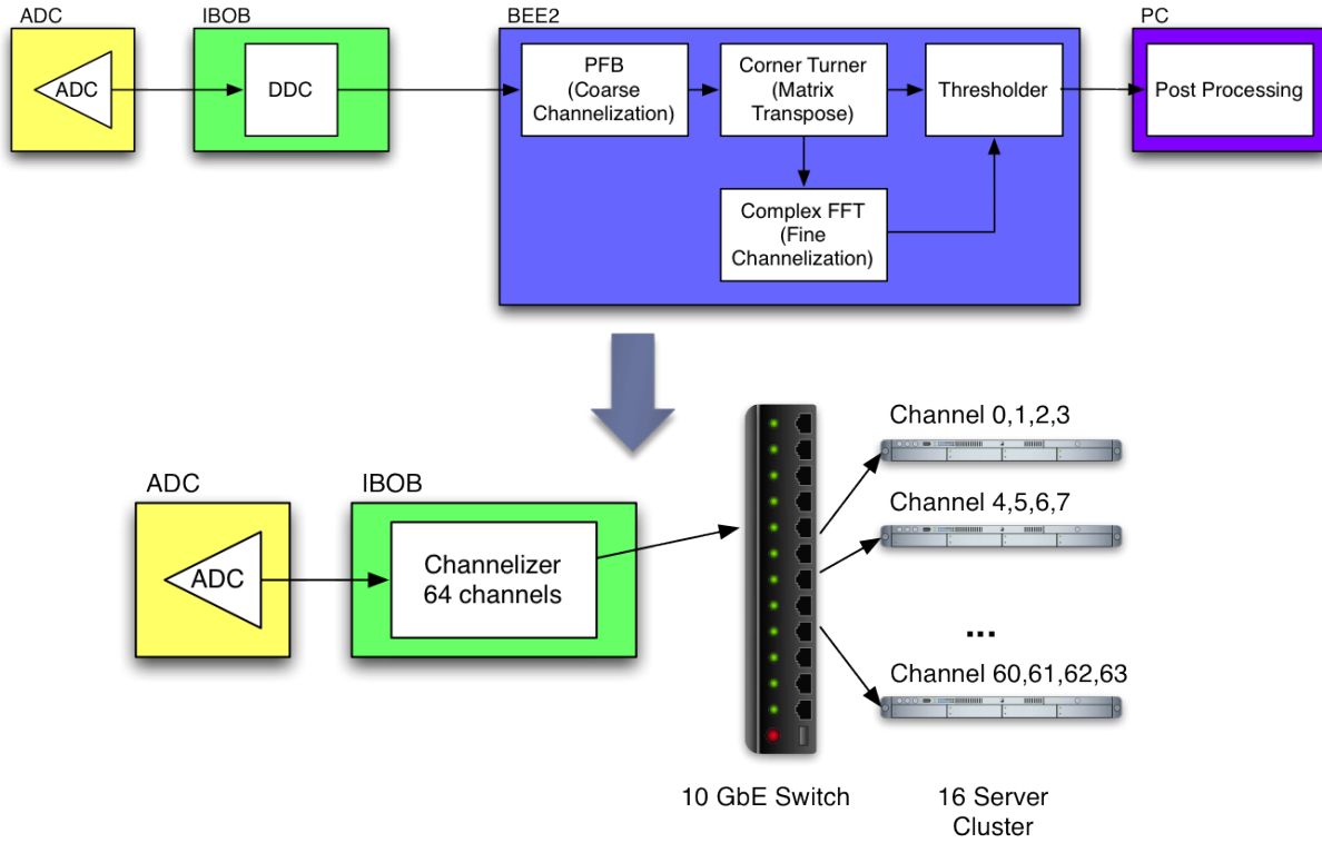
Figure 3.16: HRSS Design Based on SERENDIP V.v
