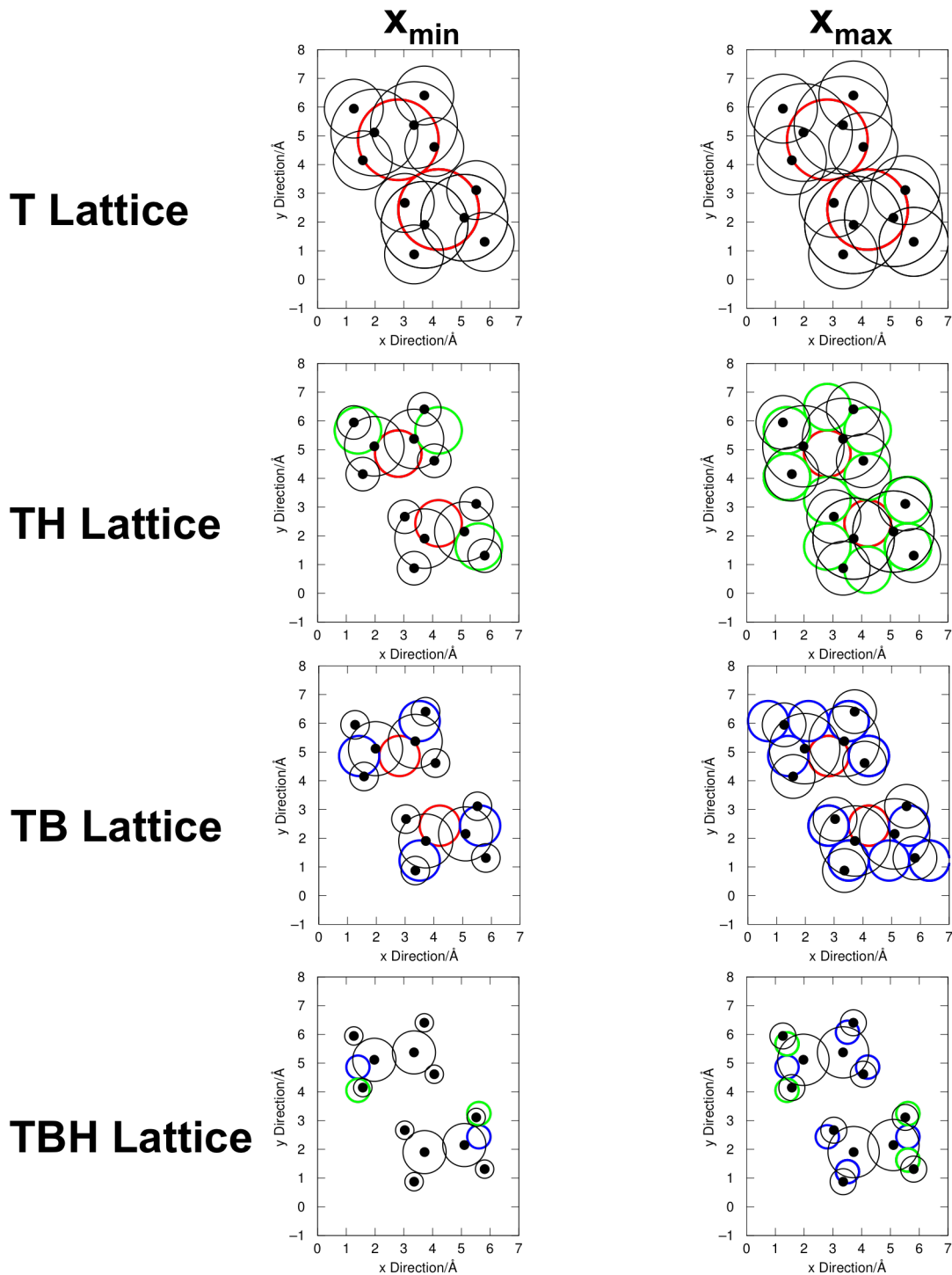
Figure 7. Illustration of pattern recognition mode (configuration 46) as a function of the atomic radii ( x \cdot R_{vdw} + (1-x) \cdot R_{cov} ) and the four different lattices. Atomic nuclei and radii are indicated as black dots and circles, respectively. Recognized top, bridge and hollow sites are given by red, blue and green circles, respectively. x_{min} and x_{max} are 0.8 and 1.0 for the T lattice, 0.3 and 0.7 for the TH lattice, 0.2 and 0.5 for the TB lattice and 0 and 0.15 for the TBH lattice, respectively.
