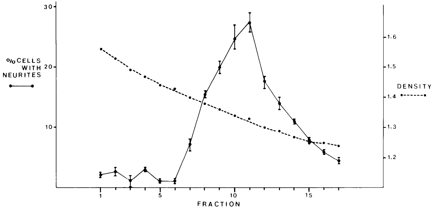
FIG. 7. Isopycnic sedimentation in associative cesium chloride gradient. MCM_{SF} was concentrated and centrifuged in CsCl containing 0.4 M GuHCl , as described. The densities of fractions were measured, and fractions were dialyzed and applied to polylysine substrata. Treated surfaces were washed and plated with motoneurons. After 24 hr, duplicate cultures were fixed and cells with neurites were counted. Error bars show means \pm 1 SD.
