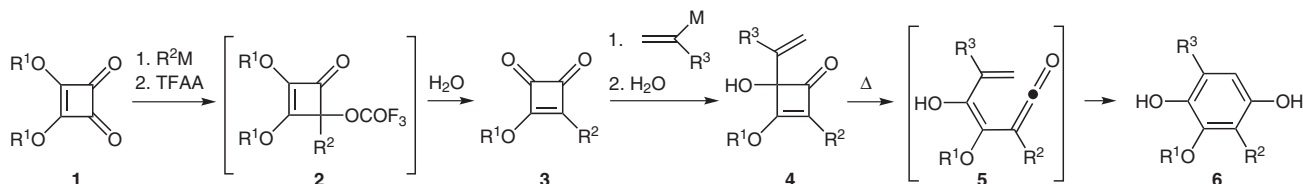
Scheme 1 Modification of squarates 1 and electrocyclic ring opening to hydroquinones 6
