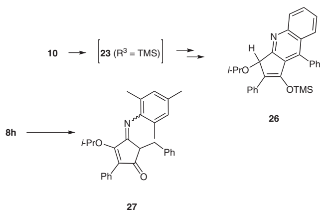
Scheme 9 Ring enlargement of 4-silyl ether 10 and of N -mesityl derivative 8h
