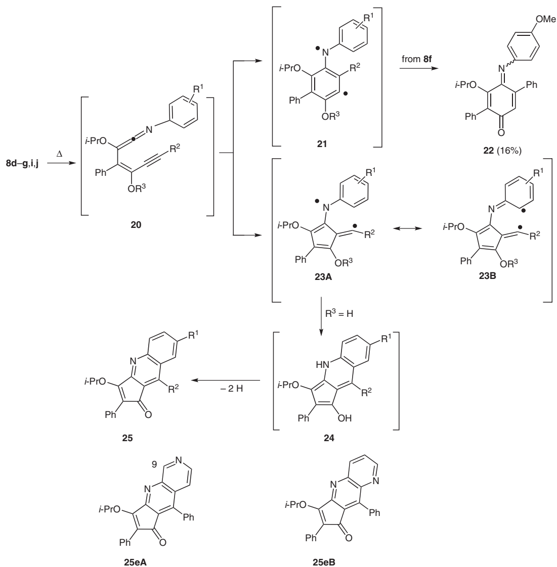
Scheme 8 Ring enlargement of 4-alkynylcyclobutenimines
