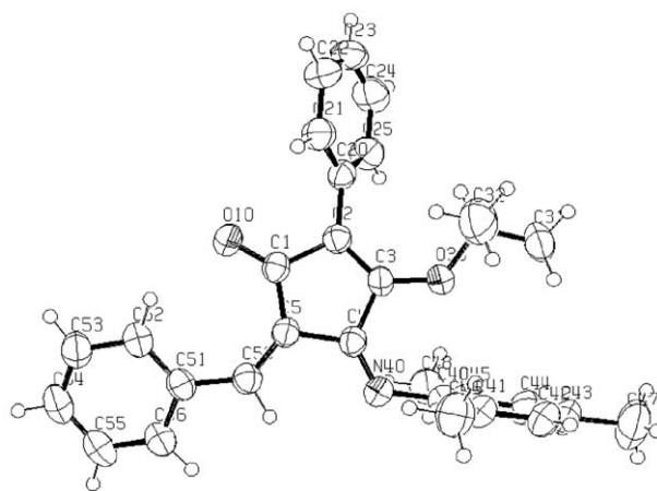
Figure 2 X-ray crystal structure of compound 27
