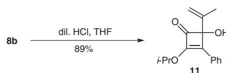
Scheme 4 Hydrolysis of iminocyclobutenone 8b
