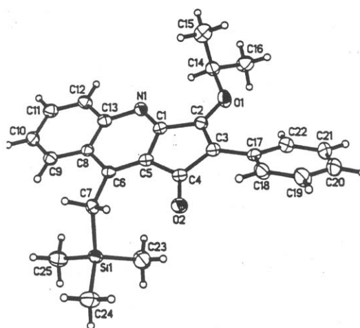
Figure 1 X-ray crystal structure of compound 25a
