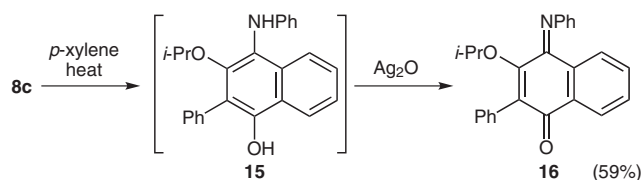
Scheme 6 Thermolysis of 4-phenylcyclobutenimine 8c
