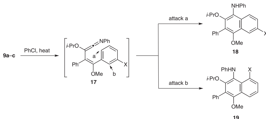
Scheme 7 Aminonaphthyl ethers from ethers 9
