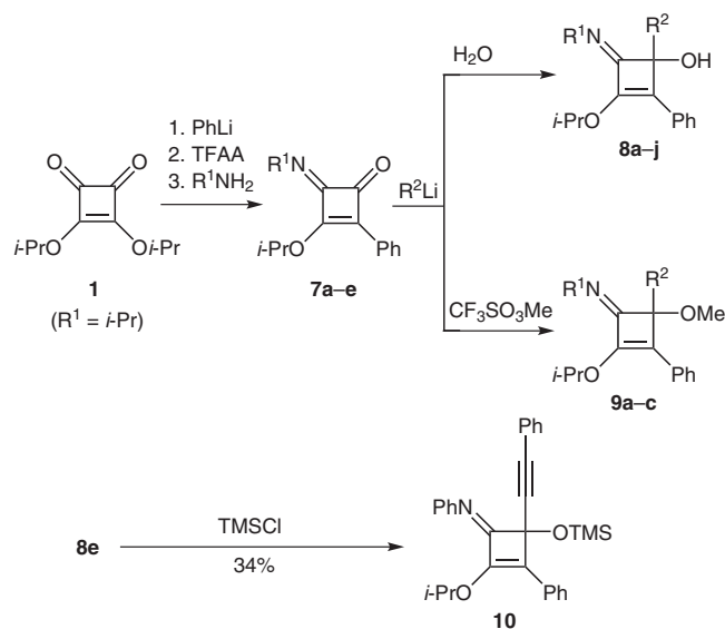
Scheme 2 Synthesis of iminocyclobutenones 7 and reaction with organometallics
