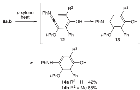
Scheme 5 Thermolysis of 4-alkenylcyclobutenimines 8a,b
