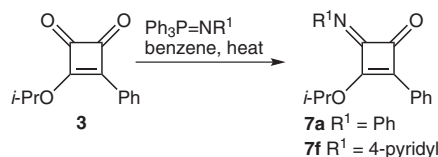
Scheme 3 Staudinger reaction of cyclobutenedione 3
