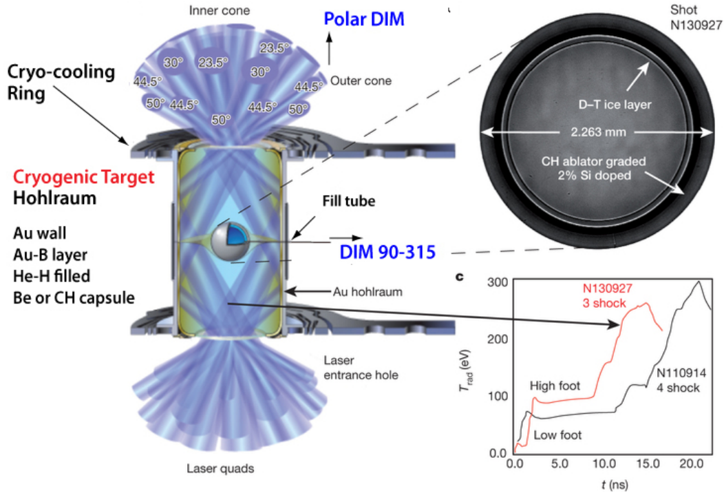
Figure 9.1: NIF hohlraum configuration for shot N130927 [96, 123].
