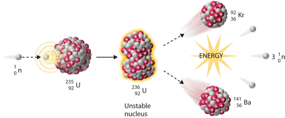
Figure 3.1: Schematic depiction of neutron induced fission depicting one possible fission fragment and neutron outcome [161].
