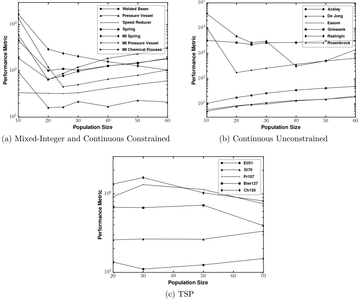
Figure 6.3: Parametric hyper-optimization results for Gnowee population size. Each algorithm and benchmark was run for 100 iterations.
