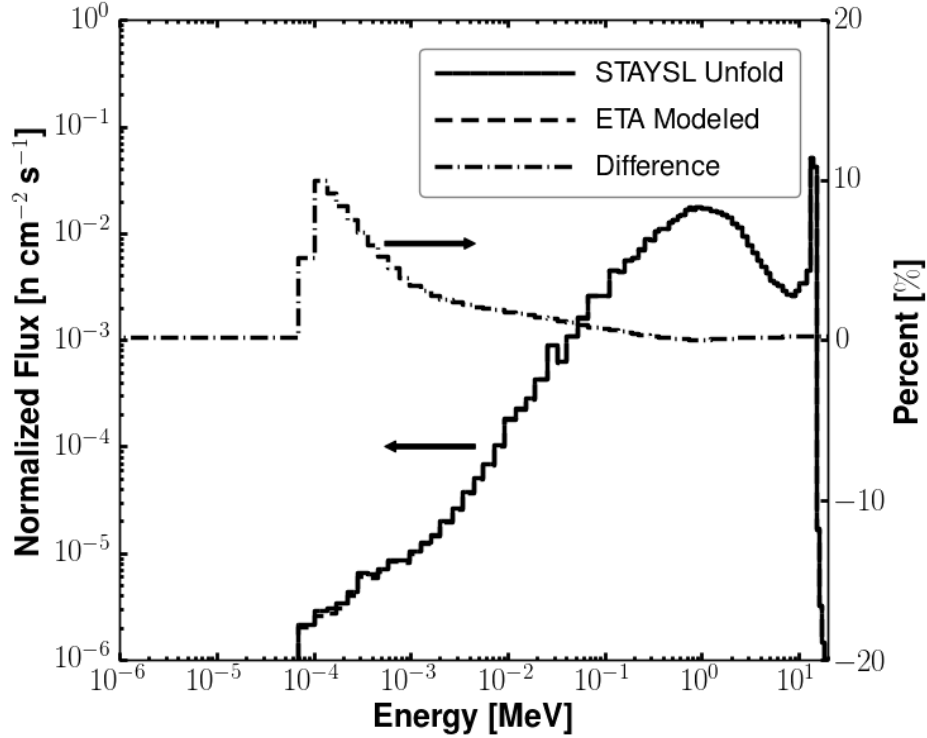
Figure 9.5: Comparison of the unfolded ETA-produced spectrum using STAYSL and the MCNP modeled objective TN+PFNS. The STAYSL unfolded spectrum is mostly beneath and indistinguishable from the ETA Modeled spectrum.
