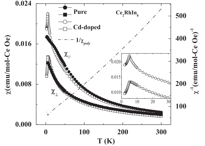
Fig. 1. Temperature dependence of the magnetic susceptibility for pure (close symbols) and Cd-doped (open symbols) \text{Ce}_2\text{RhIn}_8 , for field H = 1\text{ kOe} applied parallel \chi_{\parallel} (circles) and perpendicular \chi_{\perp} (squares) to the c -axis. The temperature dependence of the susceptibility inverse of the polycrystalline average is represented in the right axis (dashed-dot line). The inset shows the detailed Cd-doped susceptibility for low temperatures.
