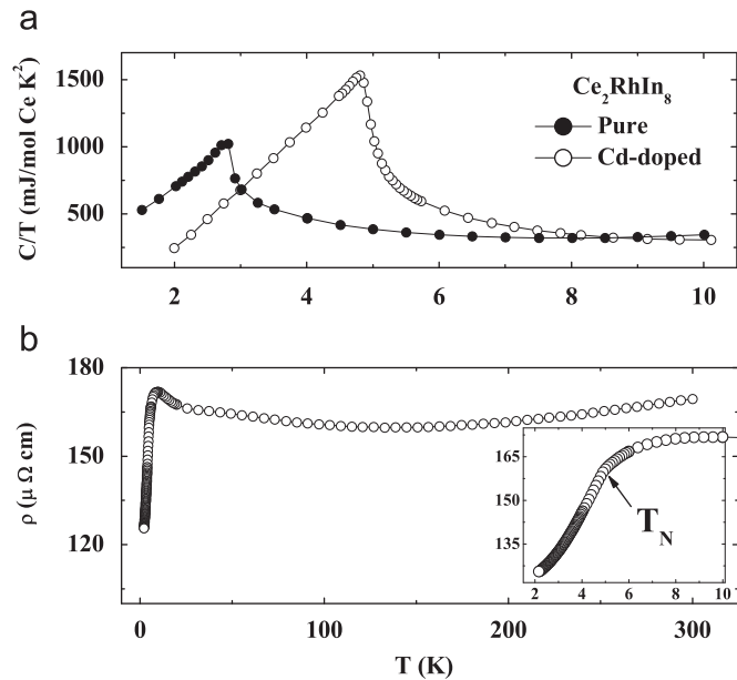
Fig. 2. (a) Specific-heat data divided by temperature as a function of temperature for pure (close circles) and Cd-doped (open circles) Ce_2RhIn_8 . (b) Temperature dependence of the electrical resistivity for Cd-doped sample. The current has been applied parallel to the ab plane. The inset in (b) point out a kink at the Néel temperature for this compound.
