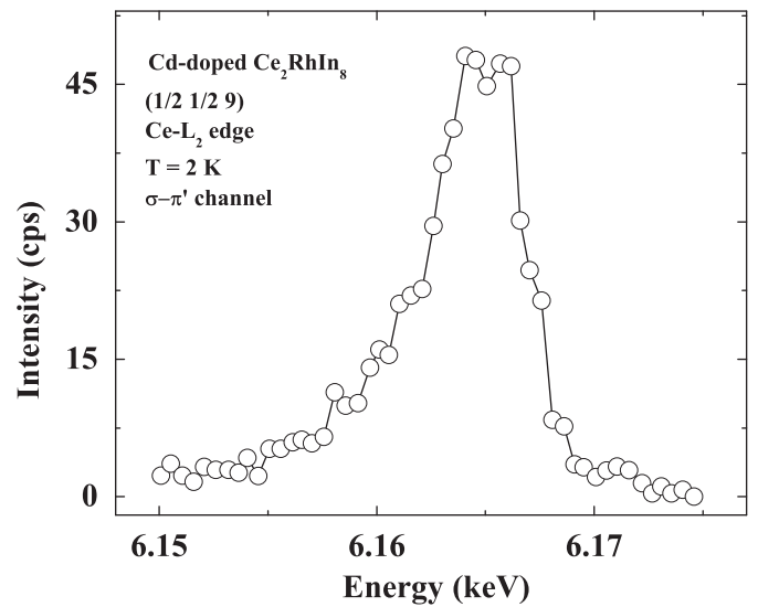
Fig. 3. Energy lineshape of the (\frac{1}{2}, \frac{1}{2}, 9) magnetic peak at T = 2 K for \sigma-\pi' polarization channel at the L_2 absorption edge of Ce. The line is just a guide to the eyes.
