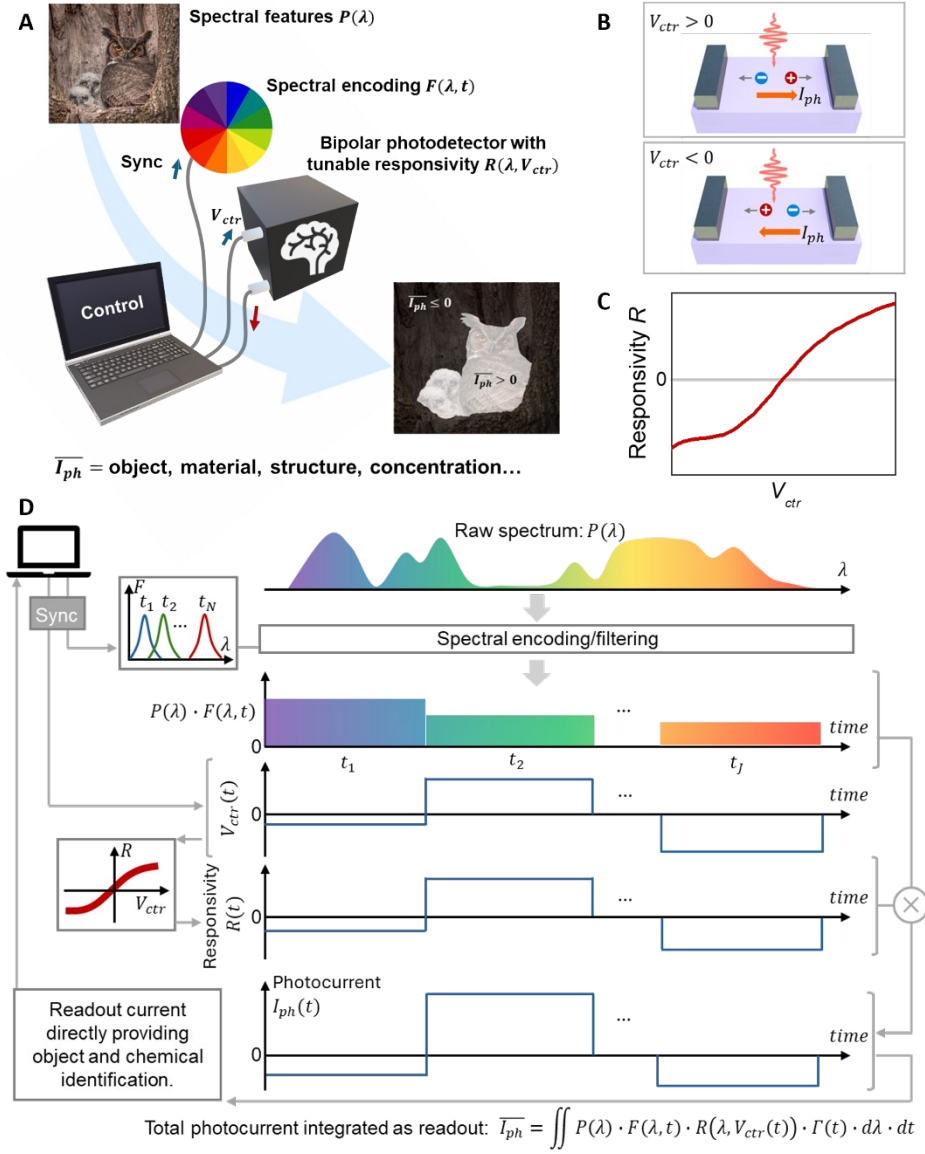
Fig. 1: Architecture of the SKM. (A) The SKM captures a scene with the synchronized operation of a spectral encoder and an electrically tunable bipolar photodetector. The device performs machine learning analysis of the scene's spectra, with the photocurrents directly as the inference results. (B) Reconfigurable computation using a tunable photodetector. Taking a photoconductor as an example, the control voltage V_{ctr}(t) can be applied as the source-drain bias to determine the photo charges' transient travel direction. (C) V_{ctr} controls both the sign and the absolute magnitude of the responsivity R(\lambda, V_{ctr}(t)) . (D) The data flow during the in-sensor computation. The object's
