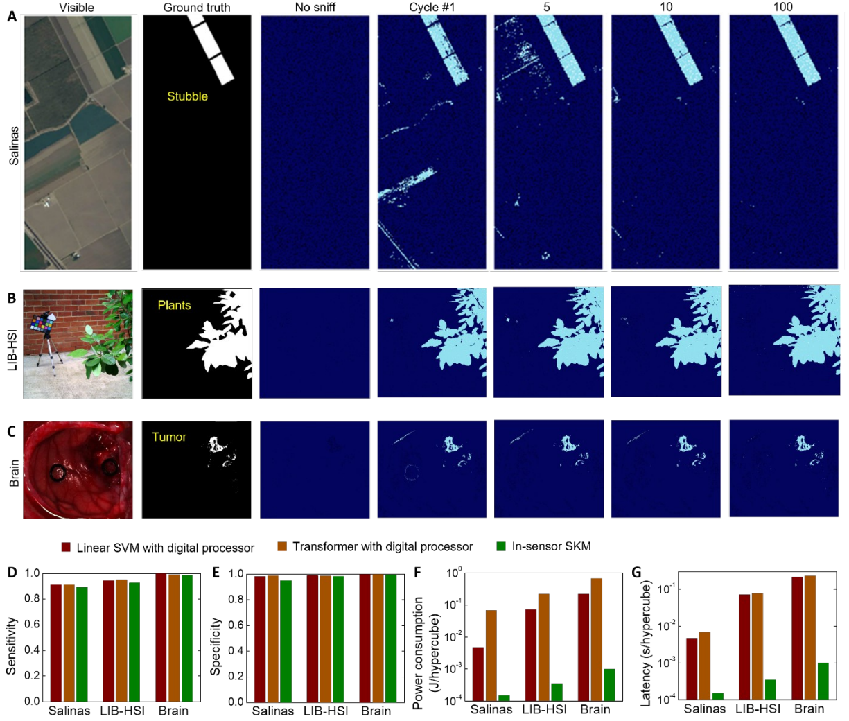
Fig. 5: Modeling of SKM architecture for complex tasks. (A) Crop identification with the Salinas Valley hyperspectral dataset. The visible image is shown on the left. The ground truth of the ‘stubble’ region is highlighted in white over a black background. Further right shows the binary classification results during gradient-blind genetic training on a simulated SKM array. White/black: training pixels identified as positive/negative. Sky blue/navy: test pixels identified as positive/negative. (B) Example RGB image and SKM identification results from a hyperspectral city scene dataset LIB-HSI. (C) Example RGB image and tumor diagnosis results from a hyperspectral human brain dataset. (D) The sensitivity of the classification results in (A)-(C), with a linear-kernel support vector machine (45) run in a digital processor, a transformer (46) run in a digital processor, and an in-sensor SKM. (E) The specificity comparisons. (F) Power consumption for capturing and processing one hypercube of each dataset. (G) The latency for capturing and processing one hypercube.
