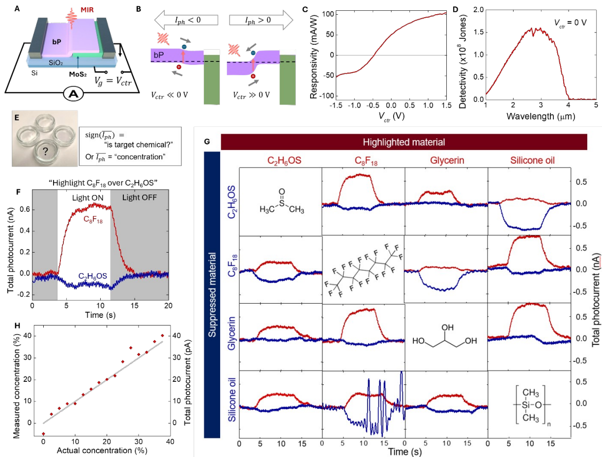
Fig. 4. MIR SKM for chemometrics. (A) Configuration of the gate-tunable bipolar bP-MoS 2 photodiode. (B) The band diagram plotted based on simulations under different gate biases. (C) The responsivity calibrated using a supercontinuum laser directed through a \lambda = 1.32 \mu\text{m} bandpass filter as the light source. (D) The detectivity calibrated with FTIR. (E) Visibly transparent analytes. (F) The total photocurrent for the C 8 F 18 sample (red line), which was highlighted ( \overline{I_{ph}} > 0 ) when the black body IR source is turned ON (white background) and drops back with IR OFF (gray background). The C 2 H 6 OS sample (blue) was suppressed so that ( \overline{I_{ph}} < 0 ) when the IR source is ON. (G) The chart for a complete set of trained binary classifications over four different chemicals in (E). Red: the highlighted materials; blue: the suppressed materials. (H) The total photocurrents, trained at 1 pA every percentage, versus the ground truth water concentration in acetone.
