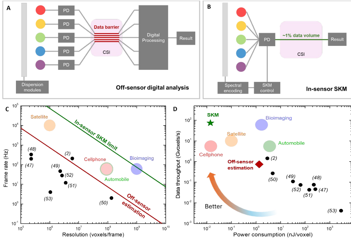
Fig. 6: Performance evaluations of the SKM architecture. (A) The architecture for hyperspectral analysis in a digital processor, with major data bottleneck at the camera serial interface (CSI). (B) The SKM bypasses the data bottleneck with in-sensor spectral information computation and compression. (C) The speed and resolution in reported works (black dots) and the ideal values for different applications (colored shades). The solid lines correspond to the estimated limits of (A) and (B) set by state-of-the-art imagers and processors (see Supplementary Text for more details). (D) Data throughput and power consumption comparisons.
