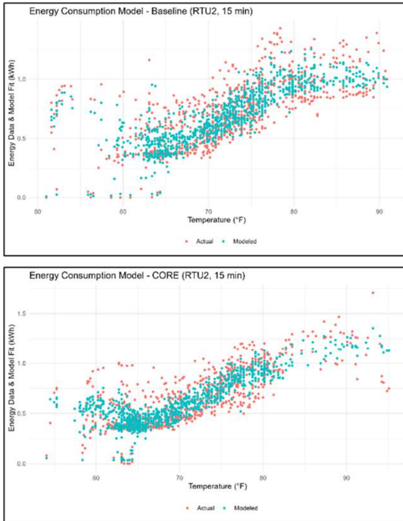
Figure 30: Measured energy vs. model-predicted energy for Baseline (top) and CORE (bottom) conditions—RTU 2—MOB-1.
