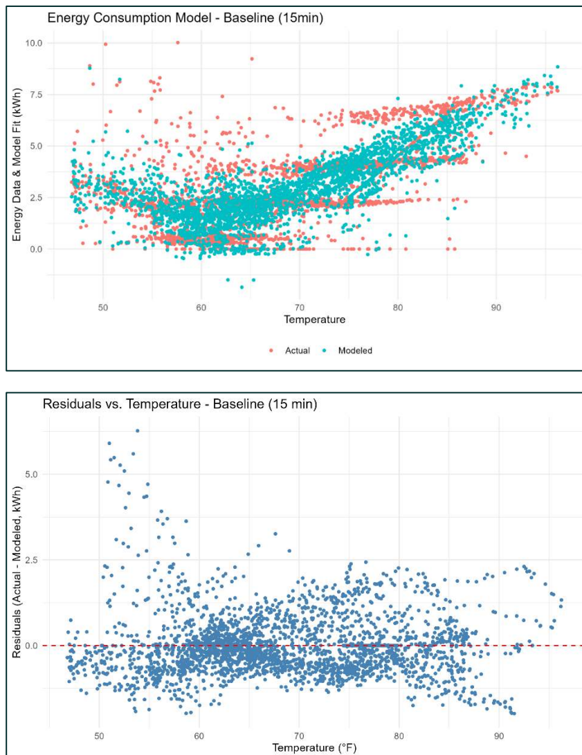
Figure 67: Measured energy vs. model-predicted energy for Baseline conditions vs. OAT (top) and Residuals
