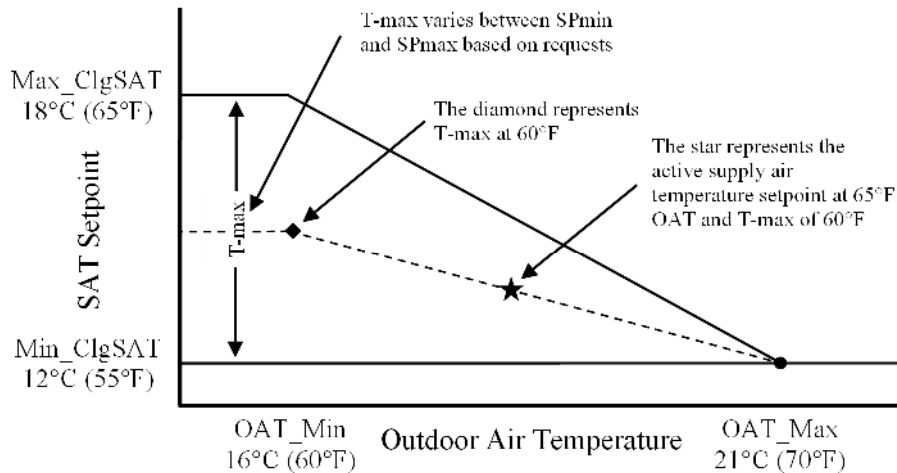
Figure 1: Example SAT reset diagram.
