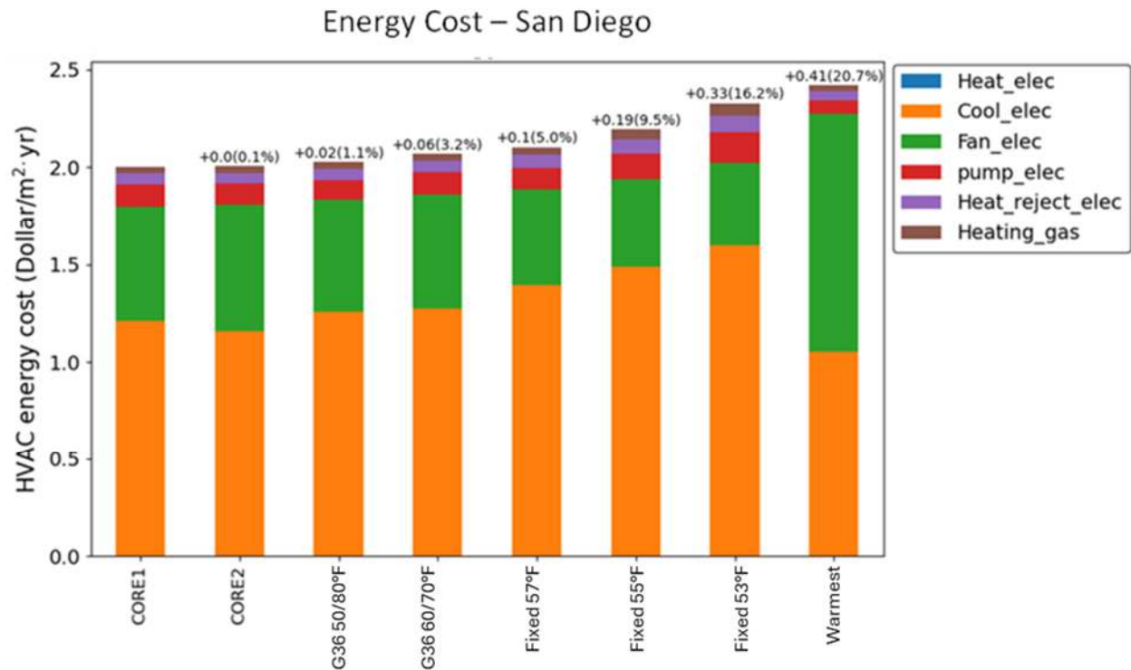
Figure 9: Energy simulation results: Total HVAC energy cost and component breakdown for San Diego climate for CORE and existing SAT control strategies.
