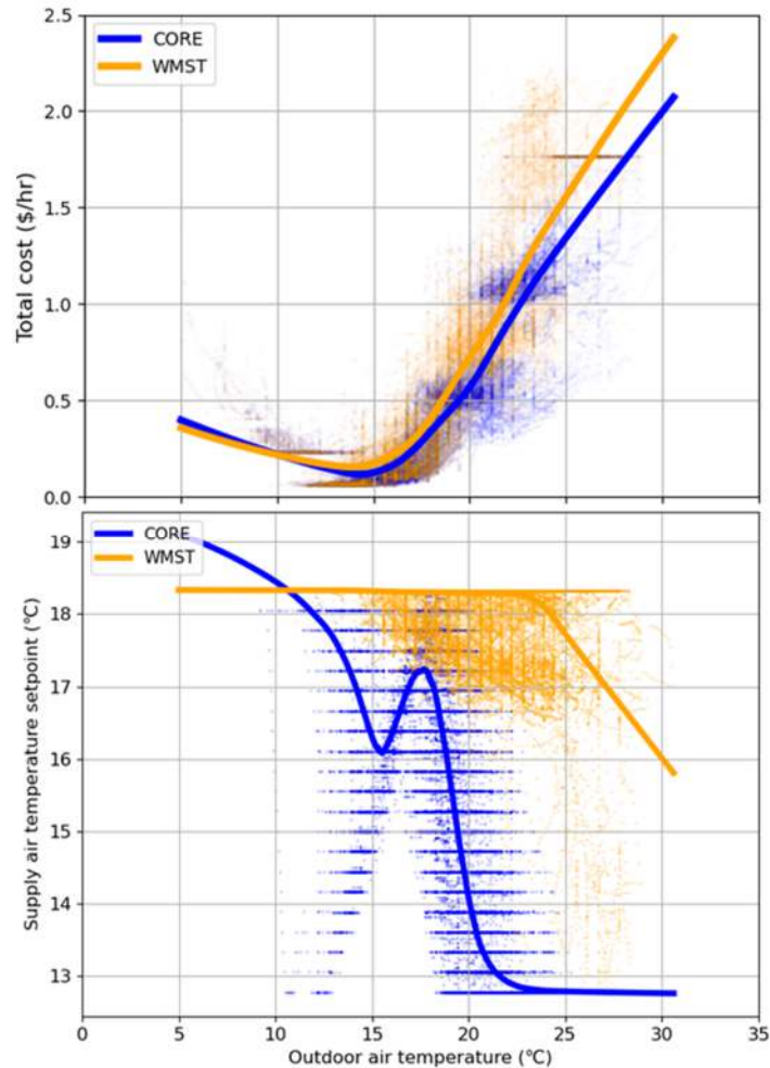
Figure 13: Scatter plots showing total HVAC energy cost and supply air temperature vs. OAT between CORE 1 (CORE) and Warmest (WMST) for San Diego.
