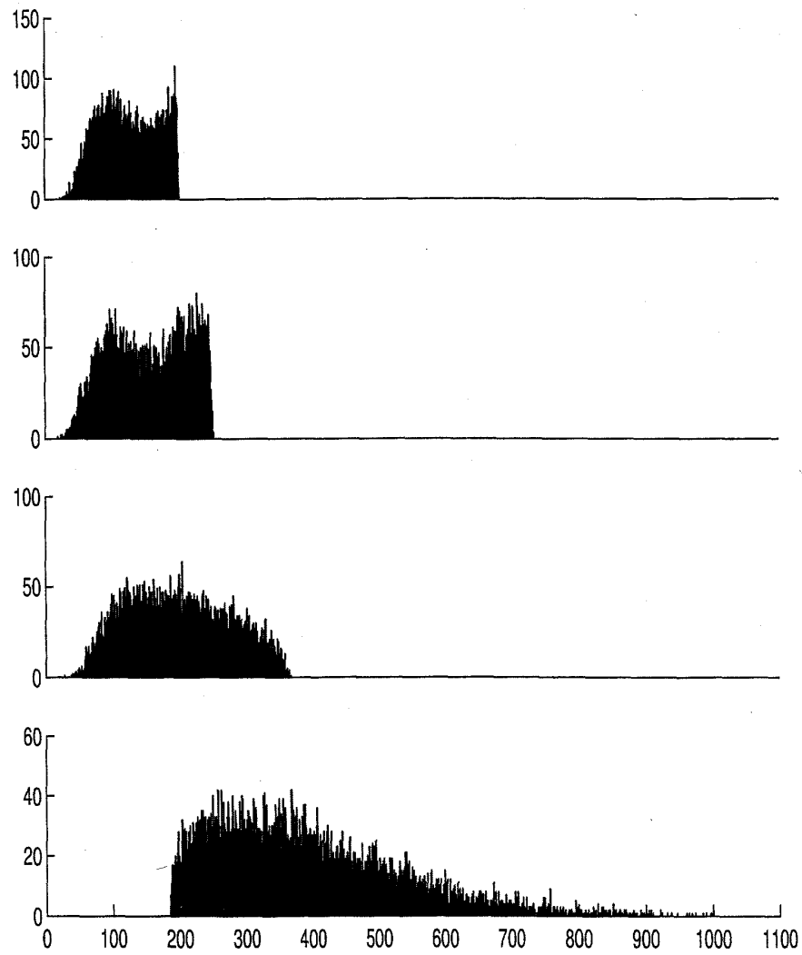
Figure 2. The Distribution of Wealth. From top down, the graph shows the distribution of the value of the optimal portfolio at time t=0.25 , 0.50 , 0.75 , and 1.00 . The initial value of the portfolio is 100. The initial value of the arbitrage A_0 is 1. The parameter values are \alpha = 1 , \lambda = 1 , and \sigma = 1 .
