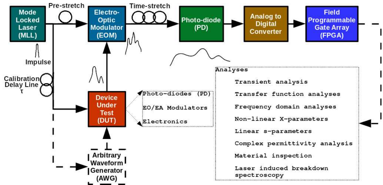
Figure 5.1: Block diagram of the Single-shot Network Analyzer (SiNA) [86].
