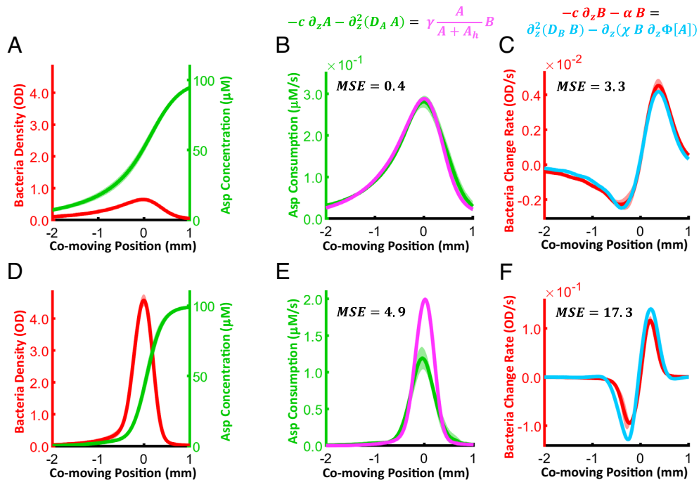
Fig. 2. The standard model for chemotaxis, the PKS model, describes the bacterial wave at low cell density but breaks down at high density. (A) The quasi-steady state profiles in the co-moving frame, of bacteria density (red) and attractant Asp concentration (green), during low cell density migration ( OD = 0.6 ). (B) Fitting the Asp dynamics of the PKS model to experimental data (above). (A and B) are the Asp concentration and the bacteria density, respectively, c is the wave speed, D_A is the molecular diffusion of Asp, \gamma is the maximum consumption rate, A_h is the half-max of the consumption rate, and z = x - ct is the coordinate in the co-moving frame ( z = 0 is defined as the peak of bacterial density). Green: LHS of the Asp dynamics equation with A and c = 4.4 \pm 0.1 \mu\text{M/s} measured and D_A = 800 \mu\text{M}^2/\text{s} (17, 18, 43–45). Throughout, uncertainty of c is the SEM. Magenta: RHS of the Asp dynamics equation with B measured, and \gamma = 0.51 \pm 0.05 \mu\text{M}/\text{OD}/\text{s} and A_h = 7.6 \pm 3.7 \mu\text{M} fit to match the LHS. The MSE between the LHS and RHS at the best-fit parameters is shown on each panel (see SI Appendix for details). (C) Fitting the bacteria dynamics of the PKS model to experimental data (above). \Phi[A] = \ln\left(\frac{1+A/K_i}{1+A/K_0}\right) is the cells' perceived signal [ K_0 \gg A and K_i = 1 \mu\text{M} (47–49)], D_B is the effective bacterial diffusivity, \chi is the chemotactic coefficient, and \alpha = 0.4/h is the measured growth rate ( Methods ). Red: LHS of the bacteria dynamics equation with \alpha , c , and B measured. Cyan: RHS of the bacterial dynamics equation with D_B = 400 \pm 100 \mu\text{M}^2/\text{s} and \chi = 3,300 \pm 230 \mu\text{M}^2/\text{s} fit to match the LHS. (D–F) is the same as (A–C) for a high cell density wave. (E and F) magenta and cyan lines are predicted using the same parameter values for \gamma , A_h , D_B , \chi as in (B and C). Here, c = 7.7 \pm 0.2 \mu\text{M/s} . The shading represents the SD across replicates. N = 6 replicates for (A–C) and N = 4 for (D–F). Uncertainties for the RHS of each equation are not shown for clarity but were included in the calculation of the MSE ( SI Appendix ).
