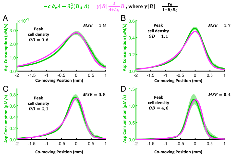
Fig. 3. Asp dynamics are consistent with cell density-dependent consumption rate. Top: modified Asp consumption rate. Green: Asp consumption rate (LHS) calculated from the data. Magenta: Asp consumption rate (RHS) with parameters \gamma_0 = 0.53 \pm 0.07 \mu\text{M}/\text{OD}/\text{s} , B_C = 5.1 \pm 1.8 \text{ OD} and A_h = 3.7 \pm 3.2 \mu\text{M} fit to match the LHS. The MSE between the LHS and RHS at the best-fit parameters is shown on each panel (see SI Appendix for details). These are shown for waves with peak bacterial cell density of OD = 0.6 (A), 1.1 (B), 2.1 (C), and 4.6 (D). The parameters were fit to all data simultaneously. The shading represents the SD across replicates: N = 6 for (A), N = 9 for (B), N = 5 for (C), and N = 4 for (D). Uncertainties for the RHS of each equation are not shown for clarity but were included in the calculation of the MSE ( SI Appendix ).
