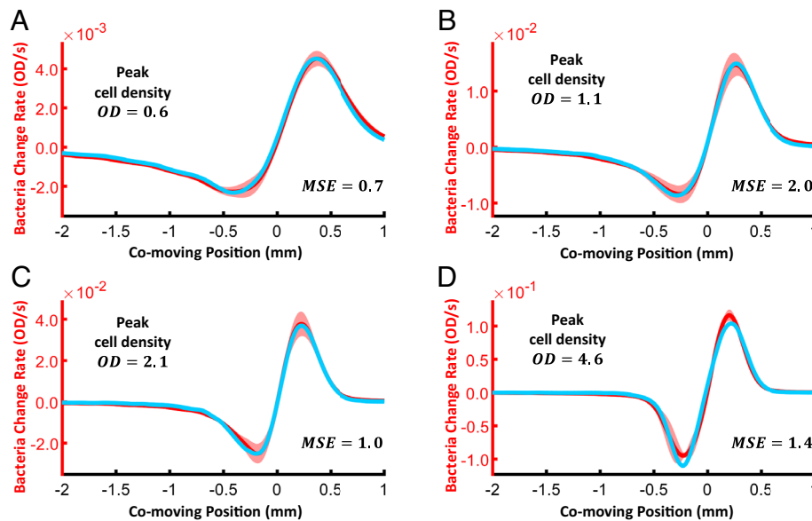
Fig. 5. Bacterial dynamics are consistent with a reduction of the chemotactic coefficient when cell density becomes large. Top: modified chemotactic coefficient. Red: rate of change of cell density (minus growth) (LHS) calculated from the data. Cyan: spatial derivative (divergence) of the flux of cell density (RHS) with parameters D_B = 440 \pm 90 \mu\text{M}^2/\text{s} , \chi_0 = 3,800 \pm 450 \mu\text{M}^2/\text{s} , B_n = 6.8 \pm 2.7 OD fit to match the LHS. The MSE between the LHS and RHS at the best-fit parameters is shown on each panel (see SI Appendix for details). These are shown for waves with peak bacterial cell densities of OD = 0.6 (A), 1.1 (B), 2.1 (C), and 4.6 (D). The parameters were fit to all data simultaneously. Uncertainties for the RHS of each equation are not shown for clarity but were included in the calculation of the MSE ( SI Appendix ).
