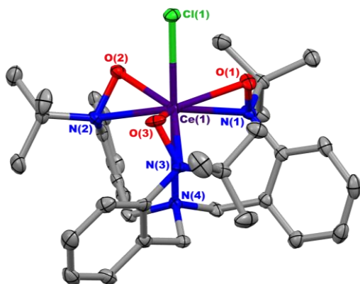
Figure 3. Thermal ellipsoid plot of 3-Cl . Hydrogen atoms omitted for clarity. Selected bond distances (Å): Ce(1)–O(1): 2.163(2), Ce(1)–O(2): 2.171(2), Ce(1)–O(3): 2.174(2), Ce(1)–N(1): 2.548(3), Ce(1)–N(2): 2.527(3), Ce(1)–N(3): 2.519(3), Ce(1)–Cl(1): 2.7436(8).
