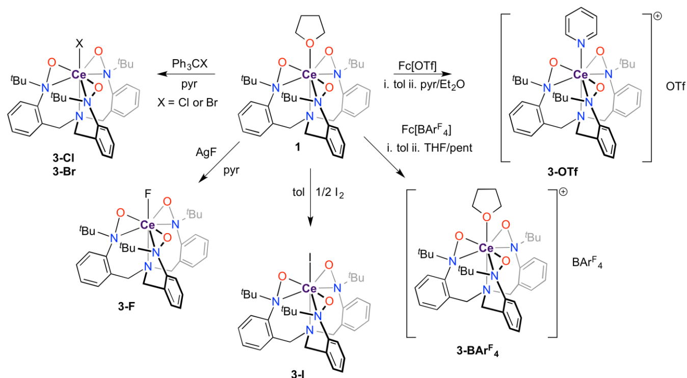
Scheme 2. Schematic of the redox chemistry performed on 1 to form the series of 3-X complexes, where X = \text{BAr}^{\text{F}_4} , OTf , F , Cl , Br , and I .
