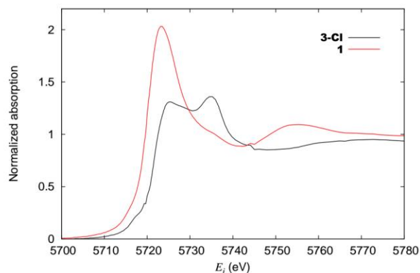
Figure 4. Overlay of the Ce L III -edge XAS spectra of 1 and 3-Cl .
