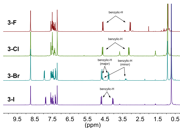
Figure 6. 1 H NMR (in d 5 -pyr) spectral overlay.
