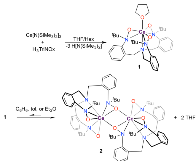
Scheme 1. Schematic of the synthesis of Ce(TriNOx)thf ( 1 ), top, and the self-association equilibrium of 1 to form [Ce(TriNOx)] 2 ( 2 ), bottom.
