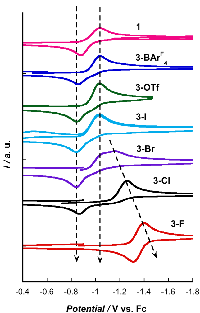
Figure 5. Metal-based Ce IV/III redox regions of the cyclic voltammograms for 1 and 3-X .
