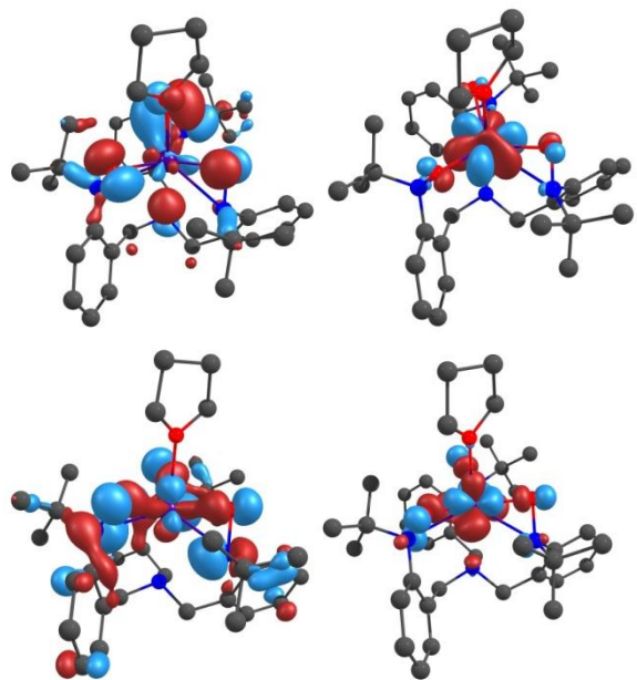
Figure 7. HOMO–12 (top left), LUMO+6 (top right), HOMO (bottom left), and LUMO+3 (bottom right) of [Ce(TriNOx)thf] + ( [1] + ), the cationic portion of 3-BAr F 4 .
