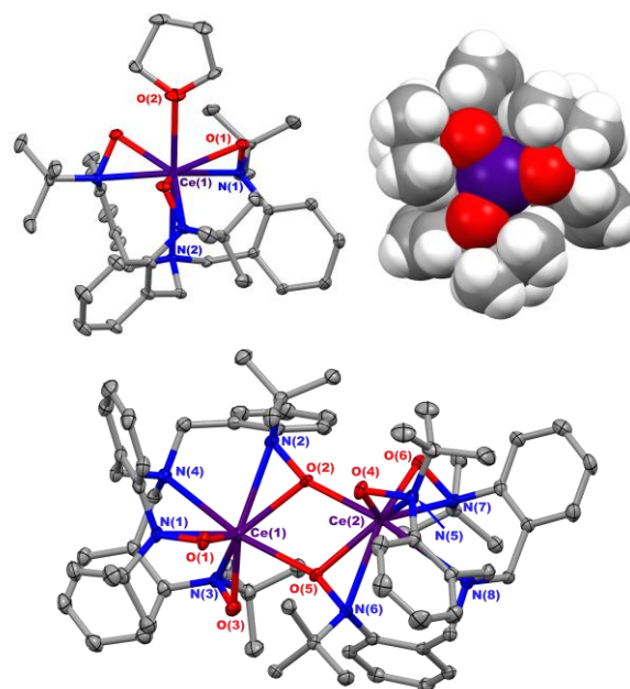
Figure 2. Thermal ellipsoid plot and spacefill diagram of 1 (top) and thermal ellipsoid plot of 2 (bottom). Hydrogen atoms omitted for clarity. Selected bond distances (Å): for 1 , Ce(1)–O(1): 2.2921(18), Ce(1)–N(1): 2.581(2), Ce(1)–O(2): 2.577(6); for 2 , Ce(1)–O(1): 2.297(3), Ce(1)–O(3): 2.273(3), Ce(1)–O(2): 2.364(3), Ce(1)–N(1): 2.639(3), Ce(1)–N(3): 2.606(3), Ce(1)–N(2): 2.689(3), Ce(1)–O(5): 2.523(3).
