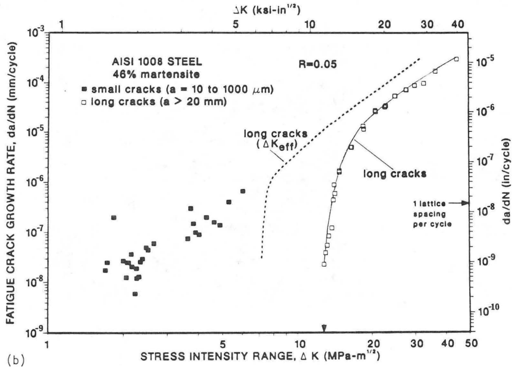
Fig. 14. Comparison of long ( \geq 20 mm) and naturally-occurring small (10 to 1000 \mu\text{m} ) fatigue crack growth in a) duplex 26 pct martensite and b) duplex 46 pct martensite microstructures in AISI 1008 steel as a function of nominal and effective stress intensity ranges ( \Delta K and \Delta K_{\text{eff}} , respectively). Note the correspondence of long and small crack data when analysed in terms of \Delta K_{\text{eff}} ( \Delta K_{\text{eff}} > \Delta K_{\text{TH,eff}} ).
