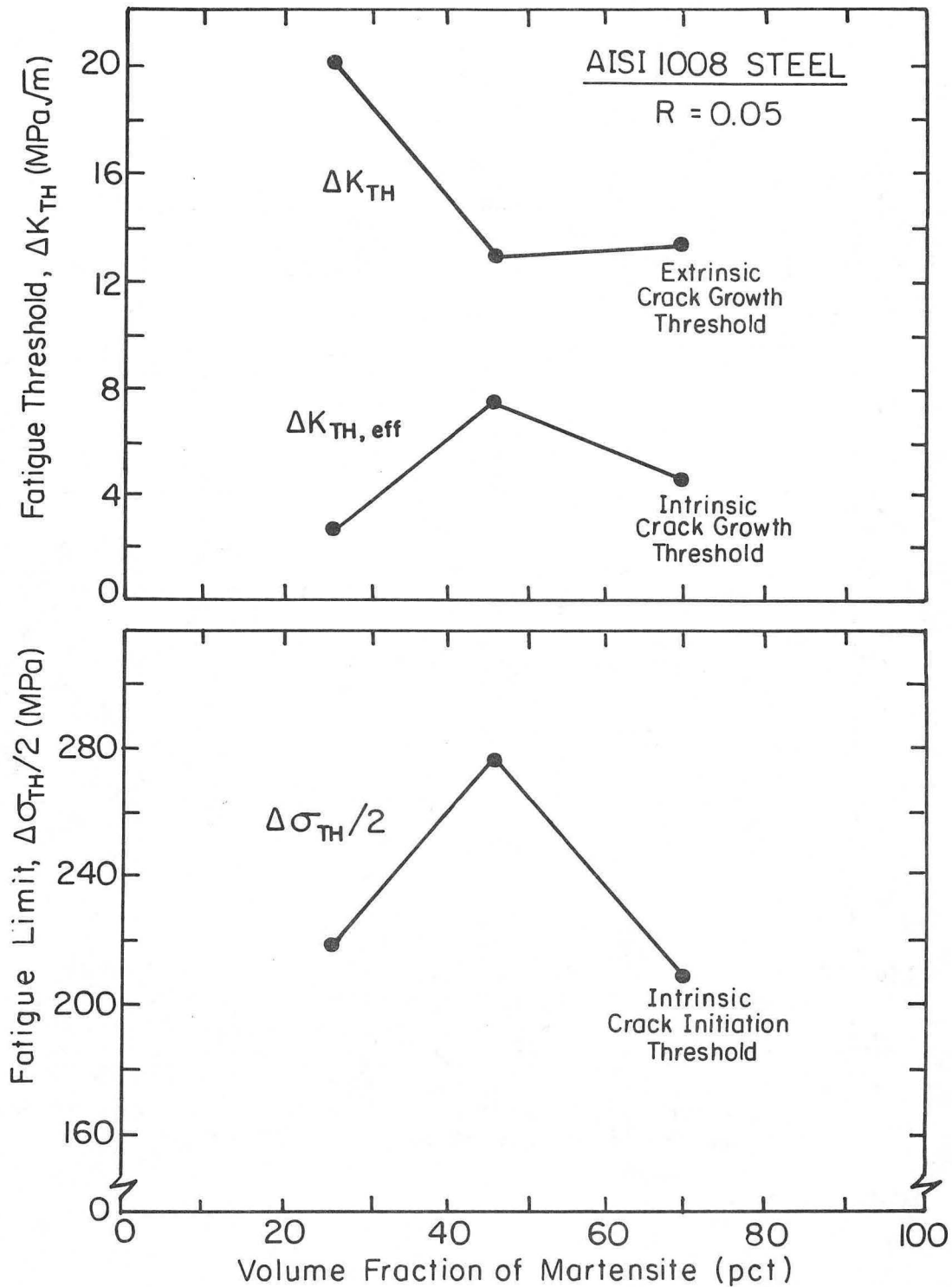
Fig. 11. Variation of nominal and effective fatigue crack growth thresholds ( \Delta K_{TH} and \Delta K_{TH, eff} , respectively) and smooth bar fatigue limits ( \Delta \sigma_{TH}/2 ) with volume fraction of martensite for duplex ferritic/martensitic microstructures in AISI 1008 steel. Note that, whereas the nominal thresholds for crack initiation ( \Delta \sigma_{TH}/2 ) and crack growth ( \Delta K_{TH} ) show opposite dependencies on microstructure, when corrected for closure the crack initiation and growth thresholds ( \Delta \sigma_{TH}/2 and \Delta K_{TH, eff} ) show similar dependencies.
