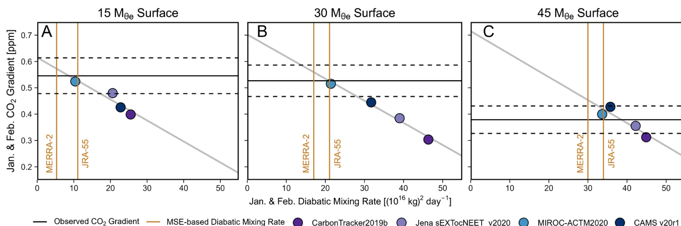
Fig. 4. Exploring the correlation between January and February ATM-based mixing rates at (A) the 15 M_{\theta_e} surface, (B) the 30 M_{\theta_e} surface, and (C) the 45 M_{\theta_e} surface and simulated atmospheric \text{CO}_2 gradients across the corresponding M_{\theta_e} surface of four transport models (3D \text{CO}_2 inversion products). Simulated gradients are from 3D concentration fields averaged at the mean dates of five airborne campaigns or subcampaigns that took place during January and February (HIPPO1, ATom2, and ORCAS1-3). The corresponding ATM-based mixing rate is calculated as the January and February average. For comparison, we show the observed \text{CO}_2 gradients (spatial bias corrected, as detailed in SI Appendix, Text S1 ) as horizontal black lines, which are calculated as the average of the same five campaigns or subcampaigns, while the dashed lines show the 1\sigma uncertainty (measurement and spatial bias correction uncertainty). We also show two MSE-based mixing rates (January and February average) as vertical brown lines. A similar figure exploring the correlation between April to November averaged \text{CO}_2 gradient and averaged diabatic mixing rate is presented in SI Appendix, Fig. S7 .
