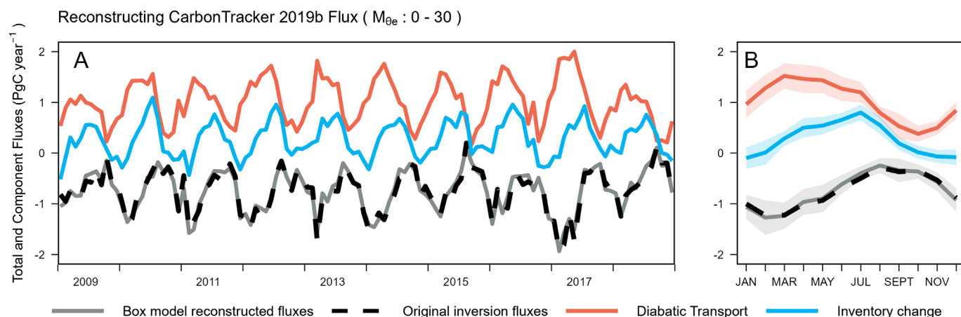
Fig. 2. (A) Monthly reconstructed air–sea \text{CO}_2 fluxes (solid gray) for the 0 to 30 ( 10^{16} \text{ kg} ) M_{0e} band (south of \sim 43^\circ\text{S} near the Earth surface) based on CarbonTracker 2019b, compared with the original monthly 3D inversion fluxes for the same M_{0e} band (dashed black). The other components (i.e., diabatic \text{CO}_2 transport and \text{CO}_2 inventory change, detailed in Materials and Methods , and Eq. 1) of the box-model reconstruction are shown as well. Positive values of the diabatic transport represent \text{CO}_2 transport into the 0 to 30 M_{0e} band (poleward transport). We note that the inventory change (blue) equals the sum of fluxes (black) and diabatic transport (red). (B) Similar to (A), but showing the flux and other components as climatological monthly averages (2009 to 2018). Shaded regions show IAV, which is calculated as the SD over 10 y for the corresponding month. We also show these reconstructions for other 3D inversion products and other surface M_{0e} bands in SI Appendix, Figs. S4–S6 .
