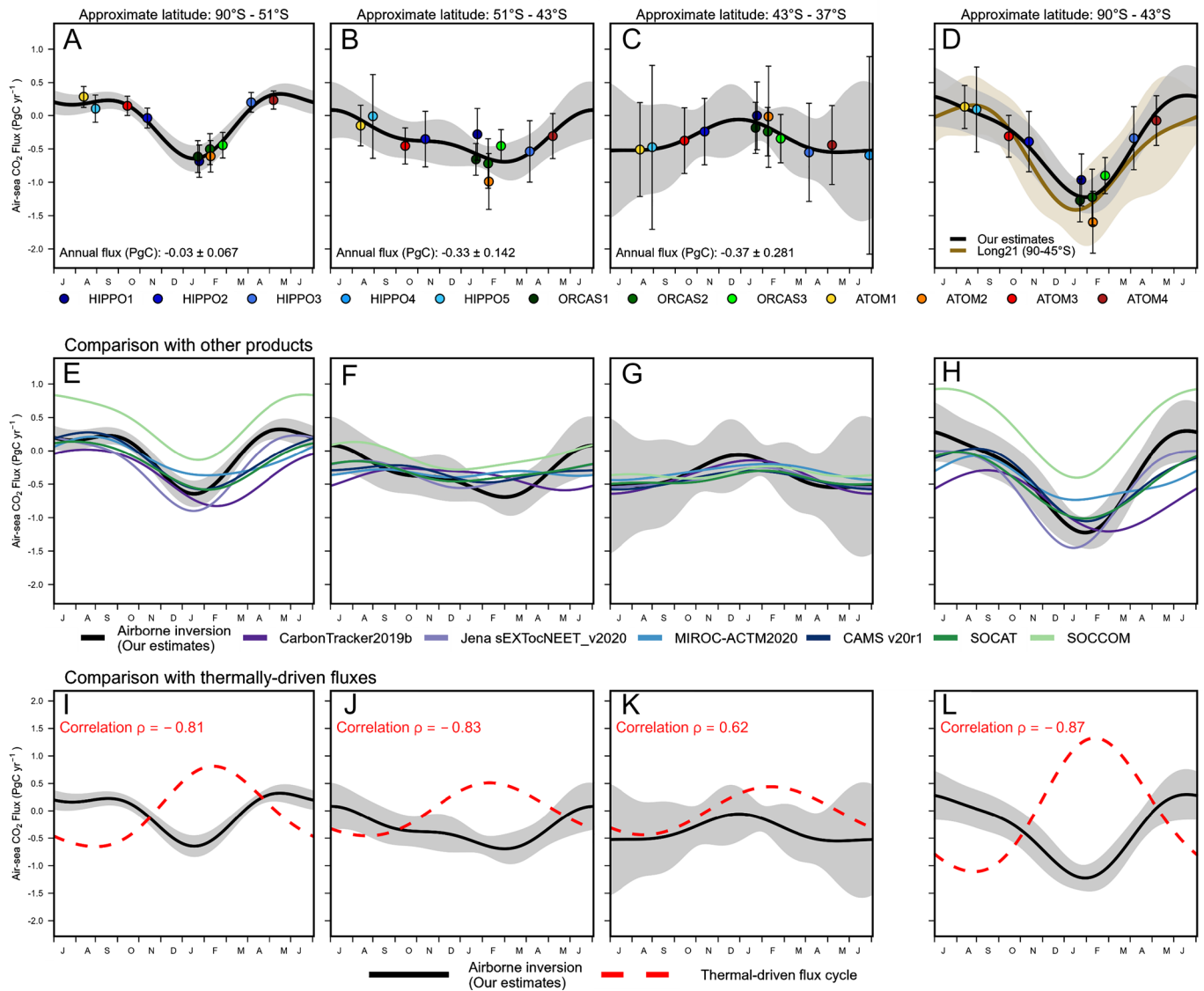
Fig. 5. (A–D) Seasonal cycle of air–sea \text{CO}_2 fluxes (negative as net oceanic uptake) estimated using the 4-box model based on airborne \text{CO}_2 observations and two sets of MSE-based diabatic mixing rates ( Materials and Methods ). Each individual point represents the calculated fluxes using airborne observations from the corresponding campaign, centering on the mean date of each campaign, while the black line is a 2-harmonic fit. Error bars represent the 1\sigma uncertainty of each flux estimate, while shaded regions represent the 1\sigma uncertainty of the 2-harmonic fits (detailed in SI Appendix, Texts S1 and S2 ). Values of air–sea \text{CO}_2 fluxes calculated for each airborne campaign transect and for each band are summarized in SI Appendix, Table S4 . Annual fluxes are from the constant term of the 2-harmonic fitted climatological flux cycles, which is equivalent to integrating the fit over a year. These approximate latitude bands (see the Top of each panel) are calculated as the zonal average latitude of the corresponding annual average (2009 to 2018) M_{0e} surface over the ocean ( SI Appendix, Fig. S2 ). We also show box-model resolved fluxes calculated using the average of six sets of mixing rates and each set of mixing rate in SI Appendix, Figs. S10 and S11 . In (E–H), we compare our estimates with four 3D \text{CO}_2 inversion products, and two neural network interpolated surface ocean \text{pCO}_2 products using SOCAT \text{pCO}_2 observations alone and SOCCOM \text{pCO}_2 observations alone. Details of these products are in SI Appendix, Text S6 . The SOCCOM product is a sensitivity run where all shipboard data from SOCAT were excluded (only SOCCOM float data were included). We note that the ocean \text{CO}_2 flux in Jena sEXTocNEET_v2020 is a prior, which is provided by assimilation of surface ocean \text{pCO}_2 observations (i.e., not neural-network derived \text{pCO}_2 ) from SOCAT (29) by the Jena mixed-layer scheme (46). The seasonal cycle of each product is calculated as the average between 2009 and 2018, except for SOCCOM, which is averaged from 2015 to 2017. In (I–L), we compare our estimates with thermally driven air–sea \text{CO}_2 flux cycles (dashed red, methods in SI Appendix, Text S3 ), which is derived from assuming 4% \text{pCO}_2 increase per degree Celsius increase in sea-surface temperature (SST) and using wind speed-dependent gas exchange. We calculate the correlation between the airborne observed flux cycle and the estimated thermal-driven flux cycle of each band. Black solid curves and shaded regions in (E–L) are corresponding airborne observed fluxes and 1\sigma uncertainty. Panels (I–L) have a different y-axis range compared to panels (A–H). We also compare our estimates with nine global ocean biogeochemistry models that are used in the Global Carbon Budget 2020 (10, 47) in SI Appendix, Fig. S9 .
