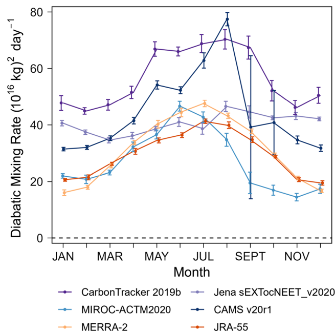
Fig. 3. Diabatic mixing rates of the 30 ( 10^{16} kg) M_{\theta_e} surface. These mixing rates are parameterized from four 3D \text{CO}_2 inversion products and MSE budget of two reanalysis products (MERRA-2 and JRA-55). Error bars represent only the IAV of parameterized mixing rates, which is shown to be small, with the exception of CAMS in September because of the close-to-zero \text{CO}_2 gradient across the 30 ( 10^{16} kg) M_{\theta_e} surface. Diabatic mixing rates of the 15 and 45 ( 10^{16} kg) M_{\theta_e} surface are shown in SI Appendix, Fig. S3 .
