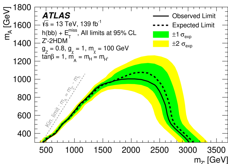
Figure 7. Exclusion limits in the Z' -2HDM model. The solid black line shows the observed limit at 95% CL, the dashed black line the expected limit. The green band gives the \pm 1\sigma_{\text{exp}} uncertainties of the expected limit, the yellow band the \pm 2\sigma uncertainties.
