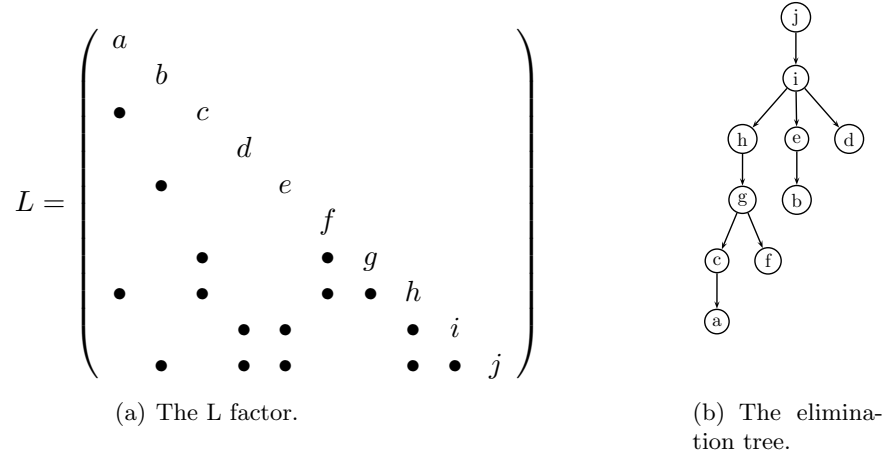
Figure 1: The lower triangular factor L of a sparse 10 \times 10 matrix A and the corresponding elimination tree.
