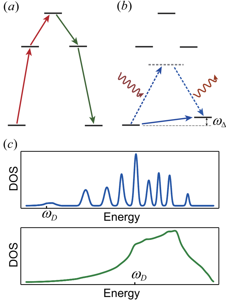
FIG. 1. (a) When the relaxation process is mediated by excitation states, Raman processes of these transitions do not yield power law dependencies, which can only result from direct tunneling between the ground state doublet as shown in (b). (c) Phonons of a SMMs system (upper) are made of acoustic phonons with very low energy and optical phonons from broadening of local vibrational modes; this difference with bulk materials (lower) brings about several peculiarities to the Raman processes in SMMs, and gives rise to the abnormalities.
