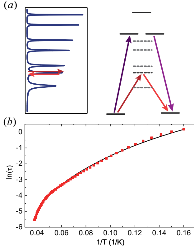
FIG. 4. (a) When the Orbach barrier is high, the vibrational modes below it collectively contribute to the Raman relaxation. (b) Summation of a series of exponential functions still leads to deceptive curves that may be mistaken as a power function. Using Eq. (1), the data (red) can be fitted with an exponent n = 3.55 .
