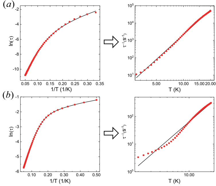
FIG. 5. (a) Fitting the data in Fig. 3(d) with \tau \propto T^{-n} and log-log scaling gives n = 7.7 ; The closeness to the standard Raman exponents may cause misinterpretation of the underlying mechanism. (b) For lower vibronic barriers, small exponents can be obtained; for instance, a barrier of 25 \text{ cm}^{-1} leads to an exponent n = 2.3 .
