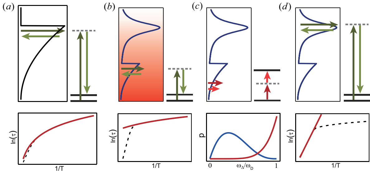
FIG. 2. (a) The conventional Raman process is mediated by acoustic phonons in solids having a large Debye energy. (b) Because of a small Debye energy, the acoustic phonons in SMM systems are well accessible for relatively high temperature, leading to \tau^{-1} \propto T^2 . (c) For SMMs with large angular momentum, the Zeeman splitting can be comparable with the Debye energy, and the double phonon process (red) can perceptibly contribute to the tunneling rate, even surpassing the Raman process (blue). (d) Raman process due to a local vibration yields an exponential dependence, which is a major cause of anomalous Raman exponents.
