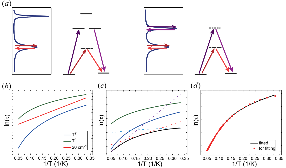
FIG. 3. (a) Two cases where small Raman exponents could be deduced from Eq.(1). (b) Exponential dependence of an energy barrier 20 \text{ cm}^{-1} is similar with \tau^{-1} \propto T^4 , and more clearly different with \tau^{-1} \propto T^7 . (c) When summed up with exponential dependence of a higher energy barrier and \tau^{-1} \propto T for the direct process, the curve (black) can be quite deceptive and easily mistaken as \tau \propto T^4 . (d) In this example, such a summed curve can be well fitted by Eq. (1) with exponent n = 4.02 .
