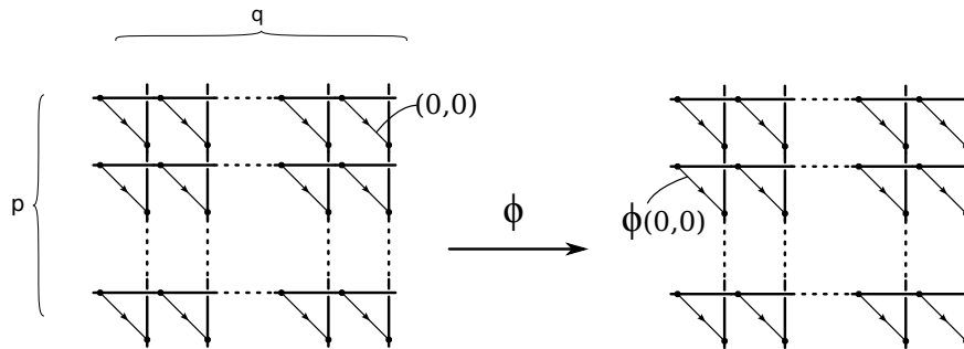
Figure 4.14: The monodromy of a (p, q) -torus knot
