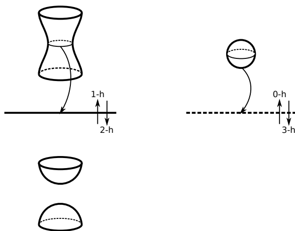
Figure 3.1: Regular fibers above and below a fold
