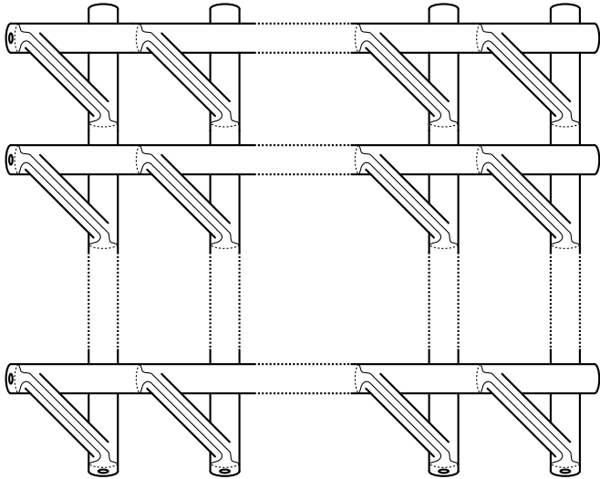
Figure 4.15: A regular fiber after adding RH, RV, RI, RII
