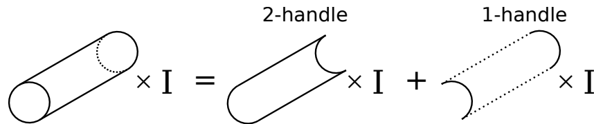
Figure 4.5: A spun-1-handle as a 3-dimensional 1-handle together with a 2-handle
