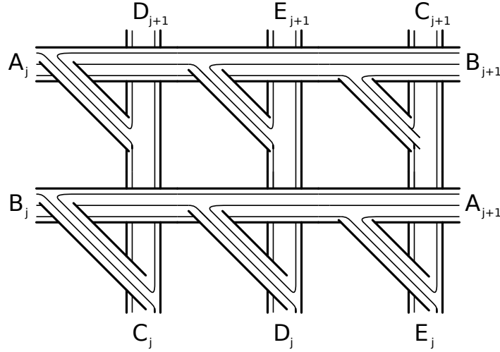
Figure 4.10: A handle decomposition of M_j^3
