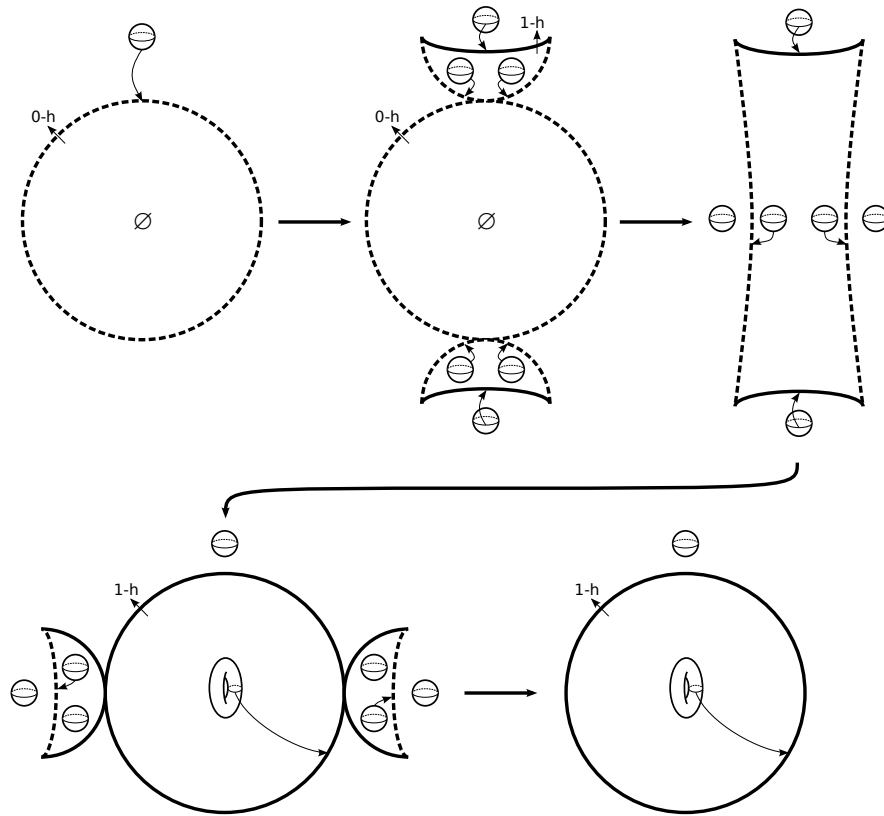
Figure 3.4: S^1 \times D as a fibration with a definite fold
