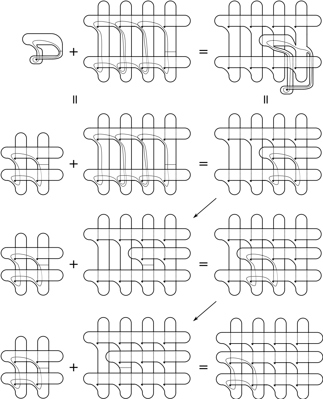
Figure 4.12: Constructing a Seifert surface of a (3,4)-torus knot
