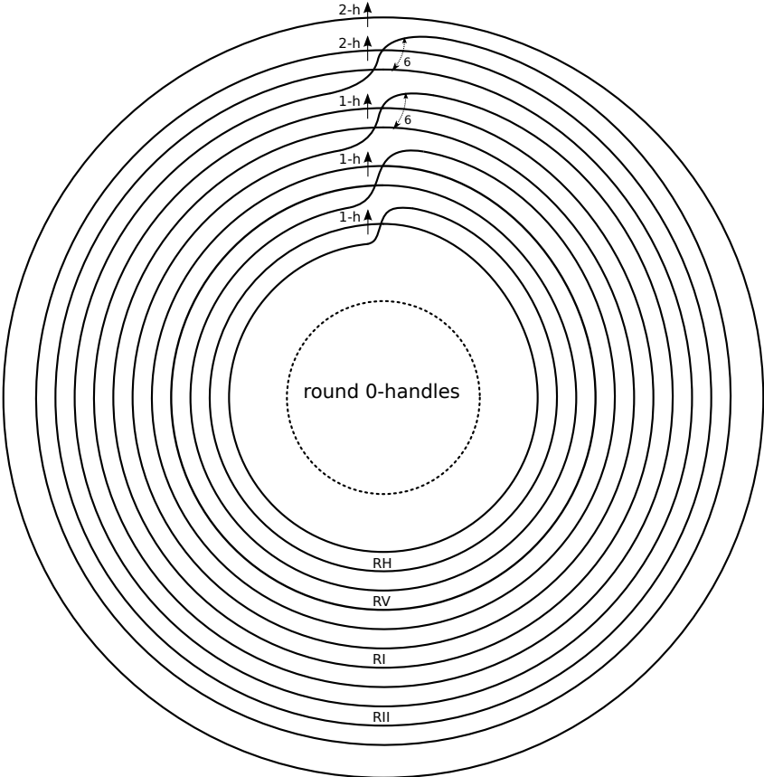
Figure 4.8: A base diagram of a BLF of X^4
