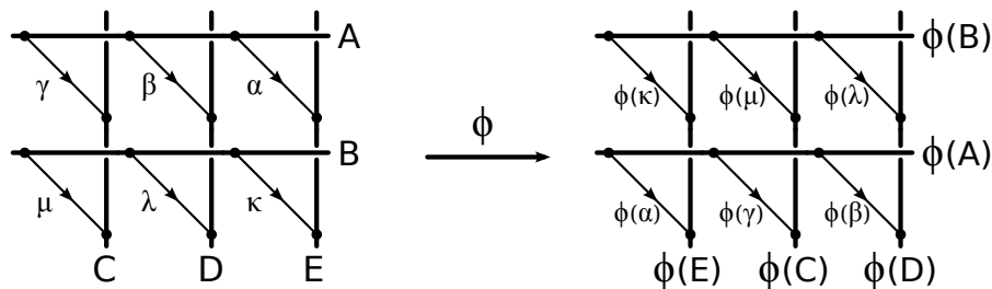
Figure 4.4: The monodromy of a trefoil knot
