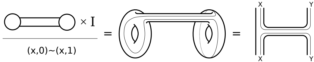
Figure 4.6: Equivalent views of a spun-1-handle
