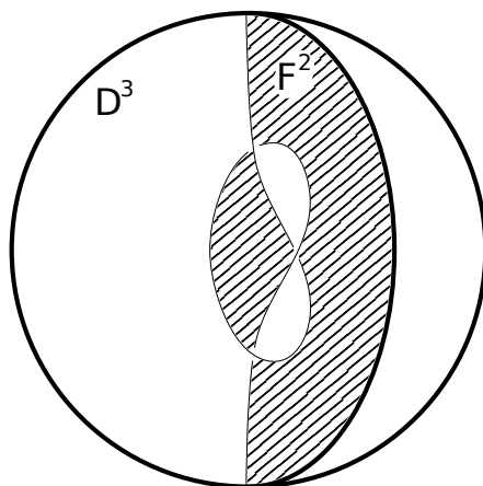
Figure 2.1: A nontrivial arc of the trefoil K embedded in D^3
