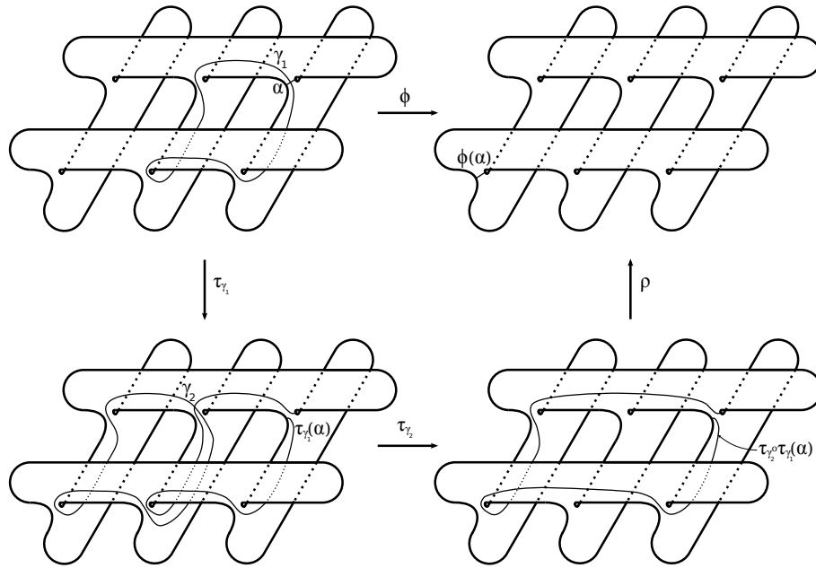
Figure 4.3: The action of two Dehn twists on \alpha
