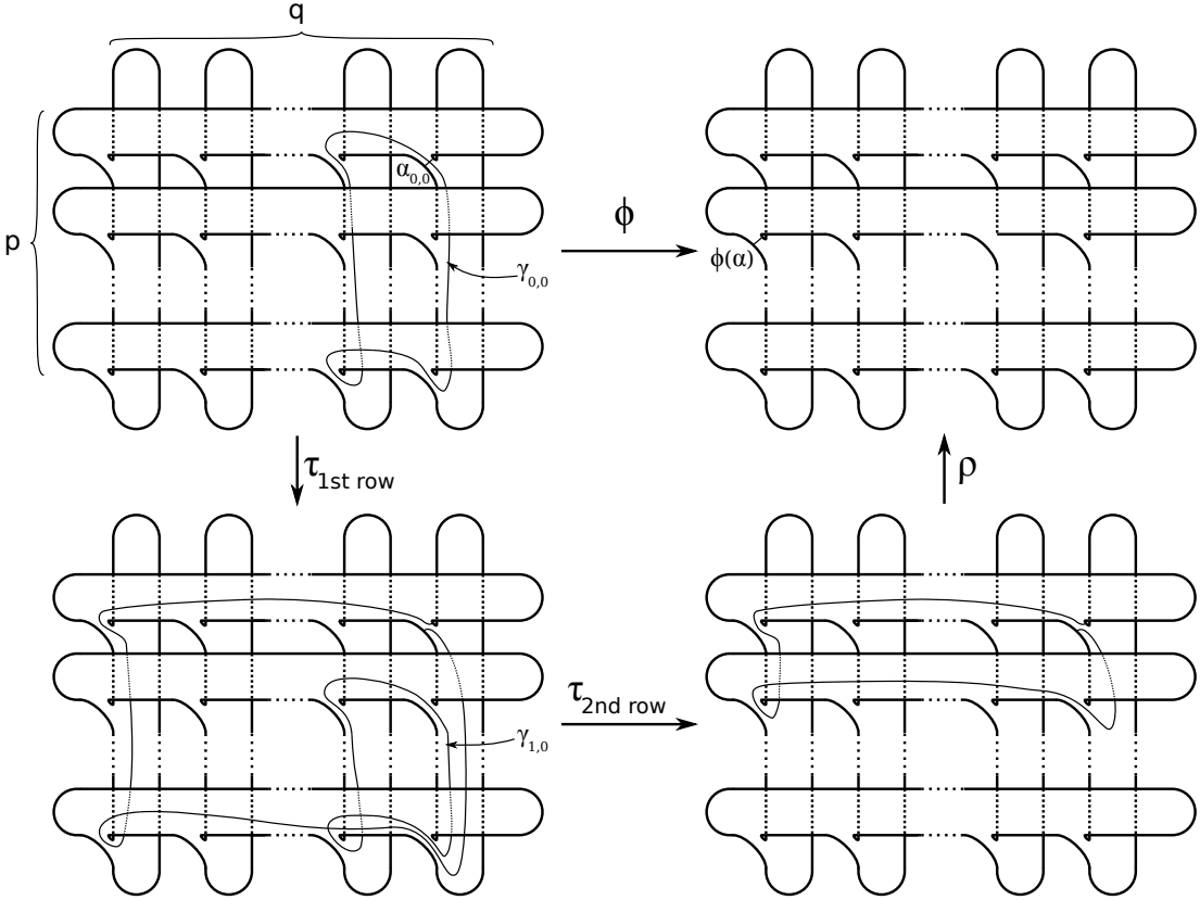
Figure 4.13: The action of \tau_{2nd\ row}\tau_{1st\ row} on the arc \alpha_{0,0}
