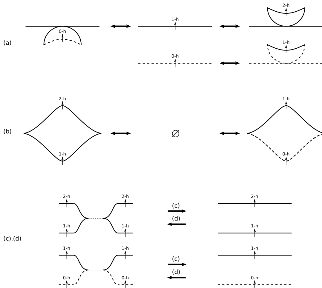
Figure 3.3: Local moves in a Cerf diagram
