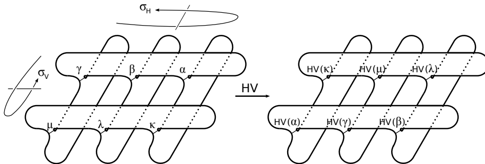
Figure 4.2: The action of HV on \overline{F^2}
