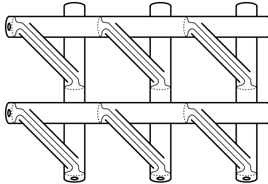
Figure 4.7: A handlebody diagram of S^1 \times \overline{F^2}
