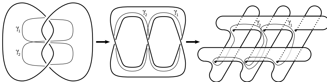
Figure 4.1: An isotopy of the Seifert surface of a right handed trefoil
