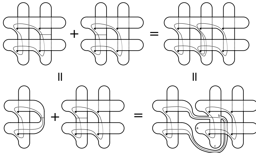
Figure 4.11: Plumbing two positive Hopf bands
