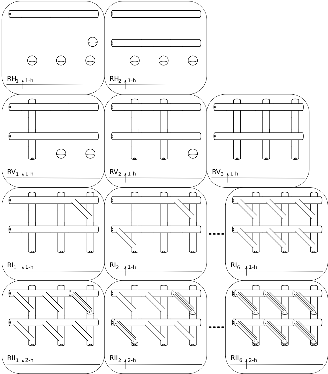
Figure 4.9: Regular fibers between various turns of the round handles RH, RV, RI, RII
