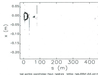
Figure 4: Transverse location of lost particles as calculated with elegant [5] (for same case as above two plots from AT).
