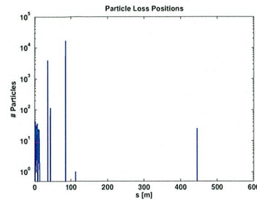
Figure 3: Loss location histogram from dark current tracking of the CD0 lattice of NGLS with a conceptual energy collimation system. Trajectories are calculated with a modified version of AT [4].
